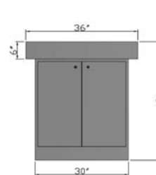
LAUNCH TABLE
