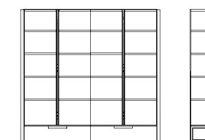
Art. CDTXL L/W 228 H 220 P/D 41 W 89.8" H 86.6" D 16.1"
