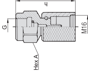
Direct Gauge Adaptor SMD20
