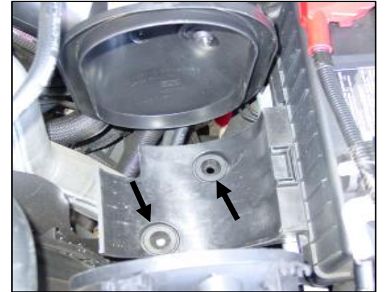
3. The factory airbox is held in place by two rubber grommets. Pull straight up and remove the box. (Note: make sure the factory grommets remain in the lower airbox support.)
