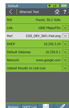
Ethernet Test Results
