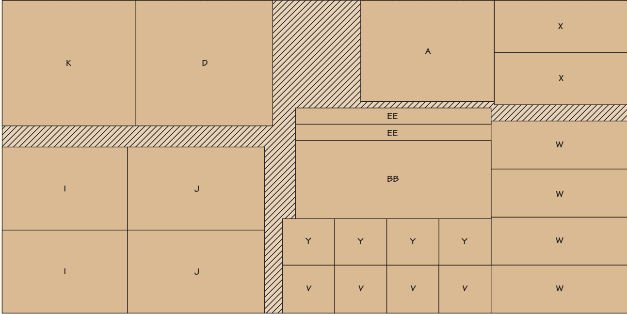
1200 x 600 x 19mm Pine Plywood
