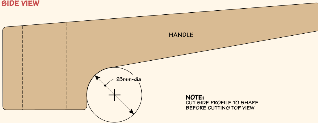
SIDE VIEW
