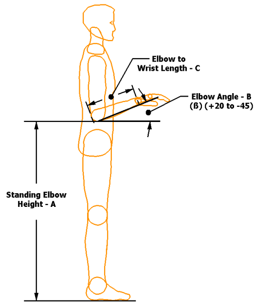
Figure 8-4. Method of combining height and tilt for input-device support surfaces
