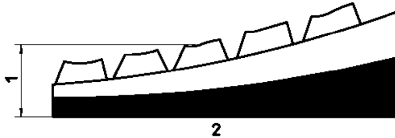
Figure 6-5. Keyboard height measured from table surface to middle of home row of keyboard. From ISO 9241, part 4 (ISO, 1998).
