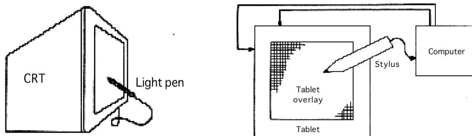
Figure 6-14. Illustrations of light pen and stylus.
