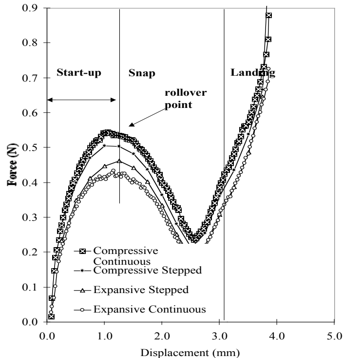
Figure 6-8. Example of force displacement curves.
