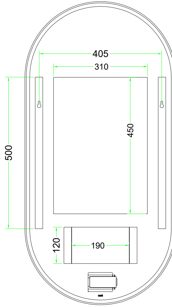
BACK VIEW
