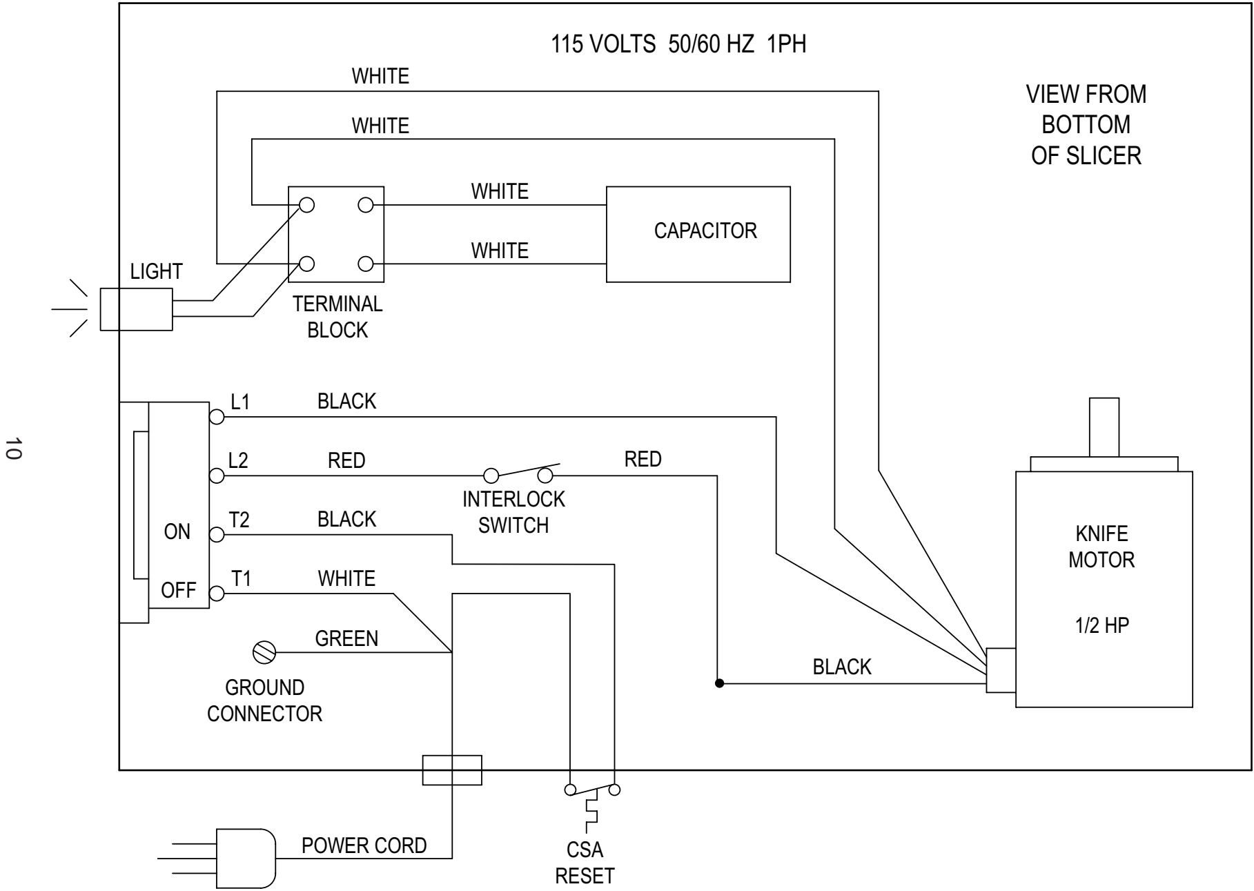
GC12D Wiring Diagram
