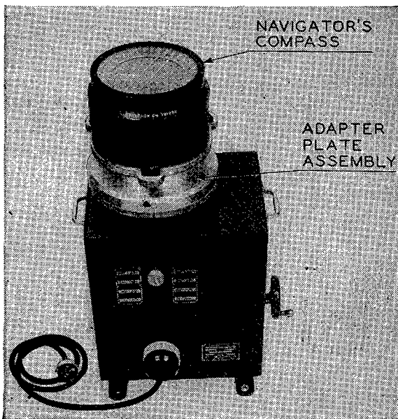
FIGURE 145.—Damping test of navigator's compass.
