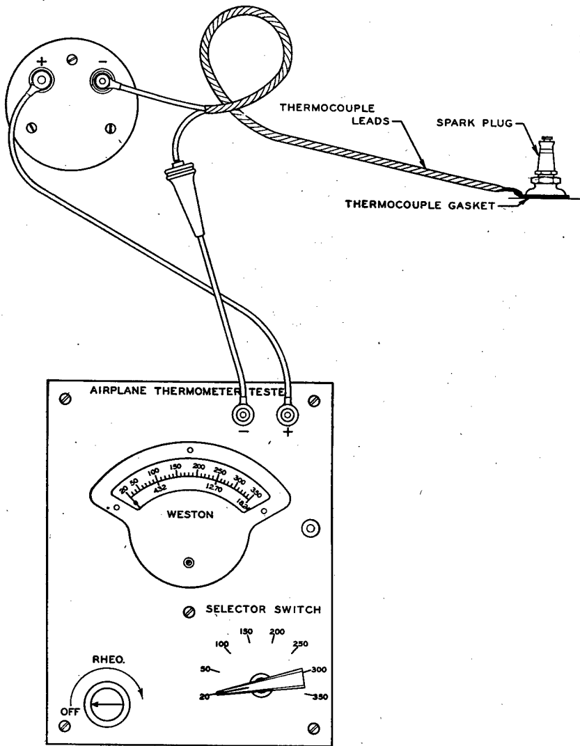
FIGURE 119.—Connection for testing cylinder temperature indicator.
