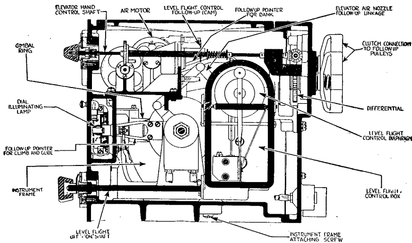
FIGURE 89.—Cross section of a bank and climb unit.
