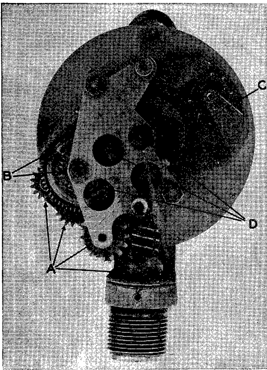
FIGURE 16.—Chronometric tachometer mechanism.
