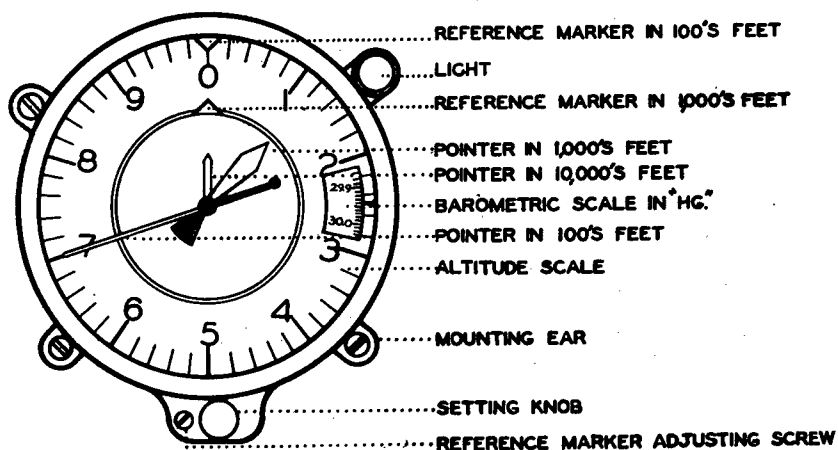
FIGURE 67.—Altimeter setting system.
