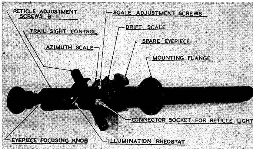
FIGURE 97.—Type B-2 driftmeter.
