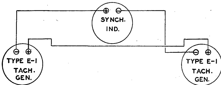
FIGURE 22.—Wiring diagram for connecting two tachometer generators with a synchronism indicator when making bench tests and shunt adjustments.
