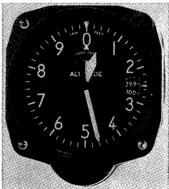
Ⓢ Sensitive altimeter.
