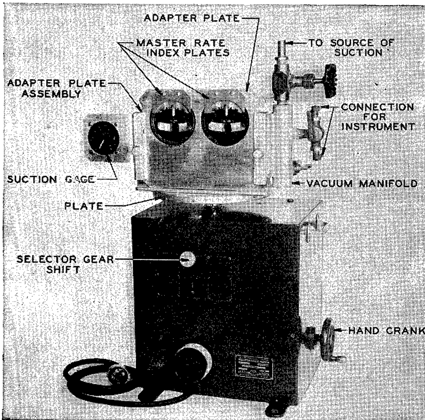
FIGURE 143.—Turntable assembly.
