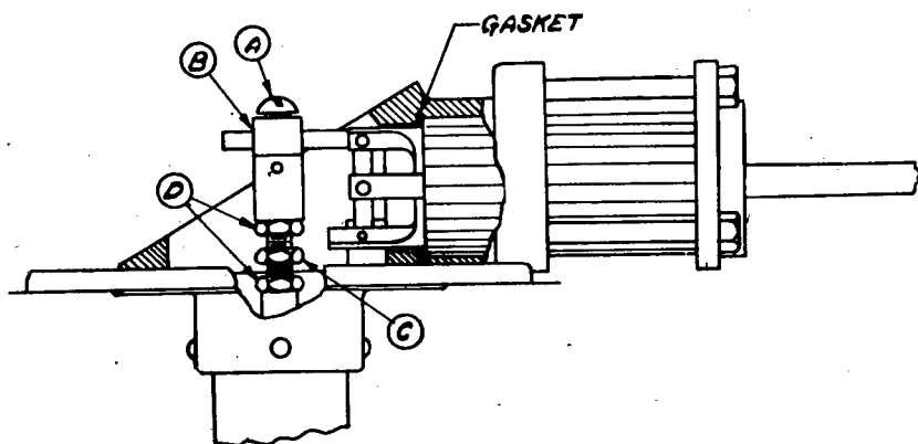
FIGURE 56.—Stroke adjustment mechanism of the hydraulically operated liquidometer.
