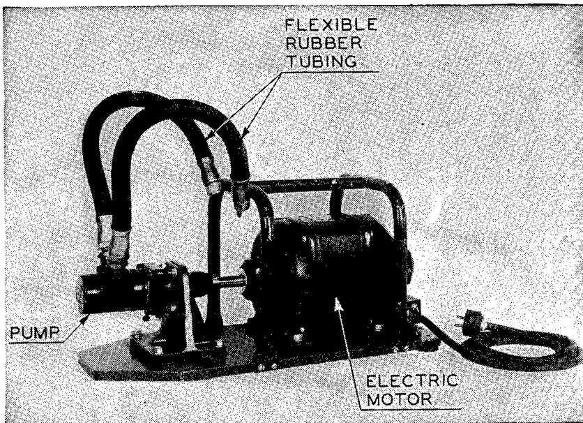
FIGURE 148.—Portable oil pump.
