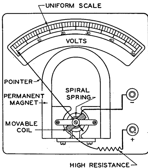
FIGURE 127.—D-c voltmeter.
