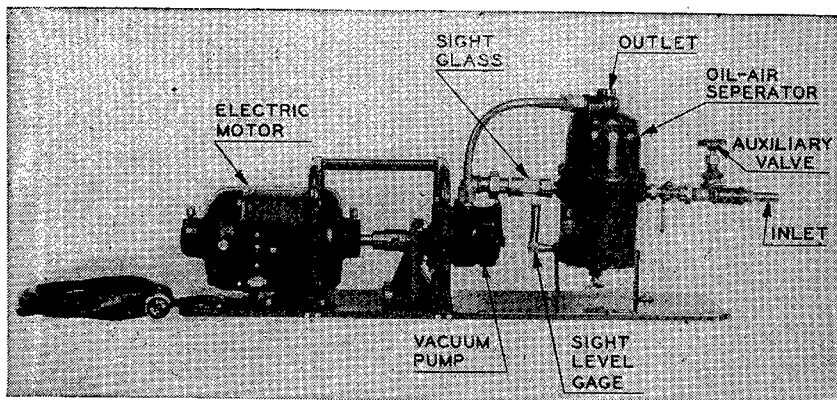
FIGURE 147.—Portable vacuum pump.
