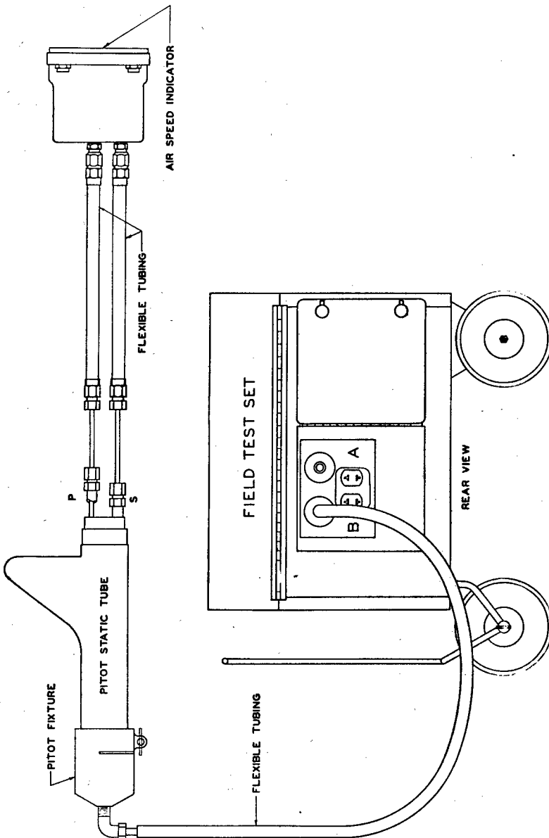
FIGURE 114.—Connection for air speed tube test (pitot fixture)
