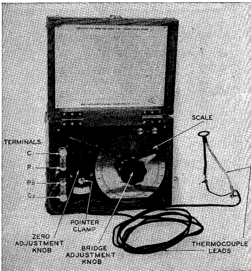
FIGURE 133.—Precision ohmmeter as used for measuring resistance.
