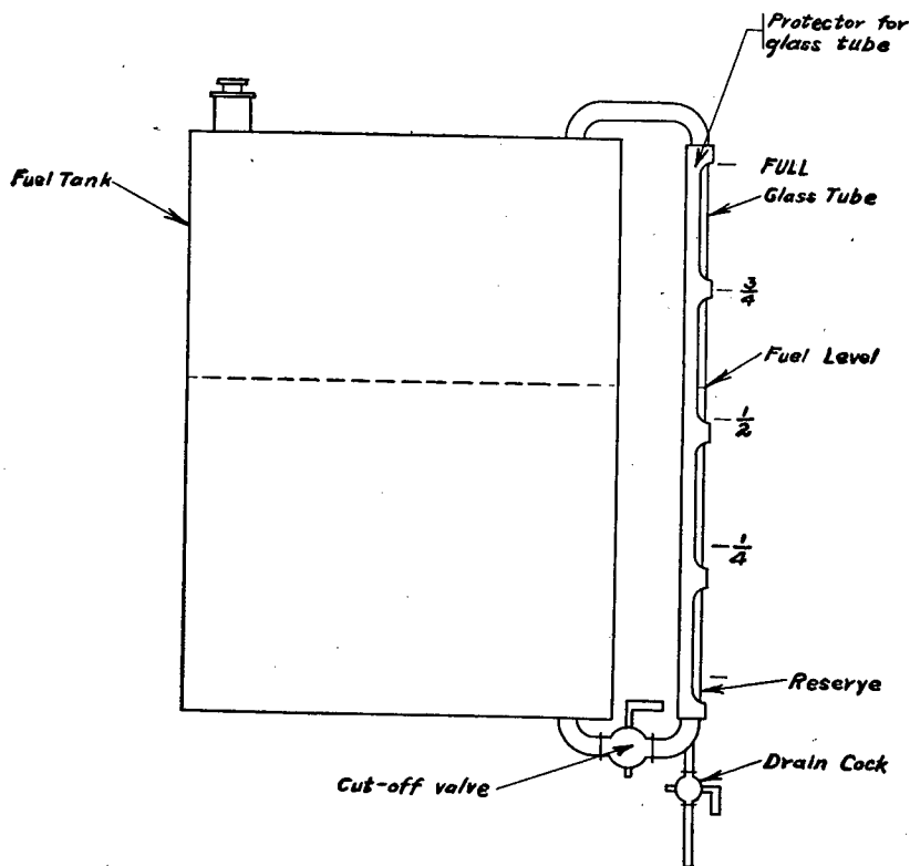
FIGURE 48.—Sight glass fuel level gage.
