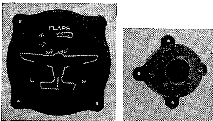
① Indicator.
