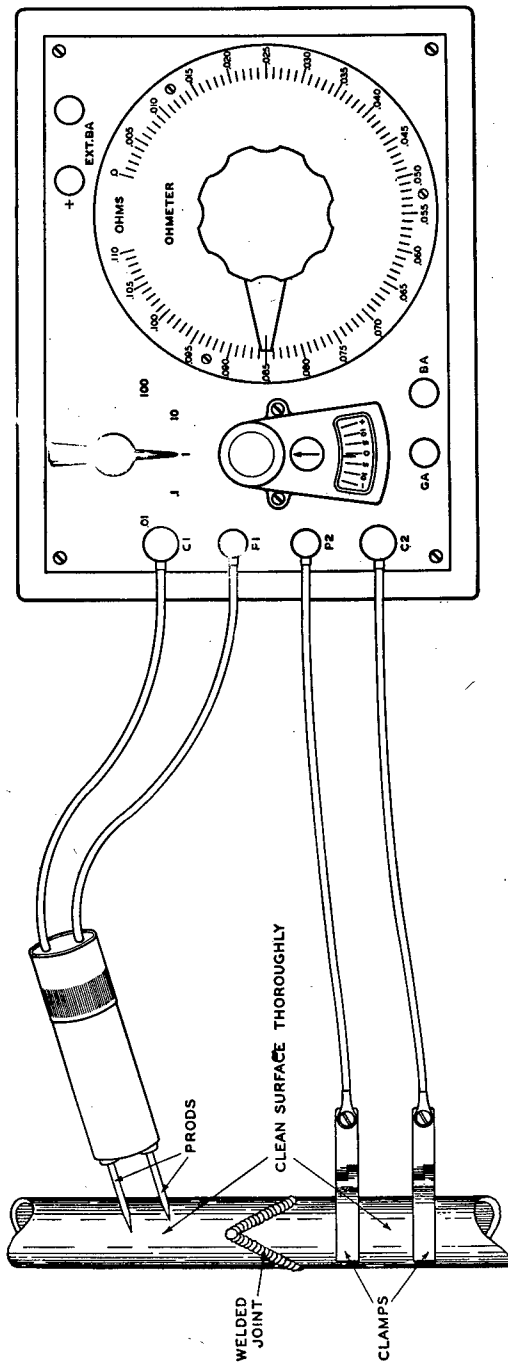
FIGURE 135.—Method of determining resistance of a welded bond with precision ohmmeter.
