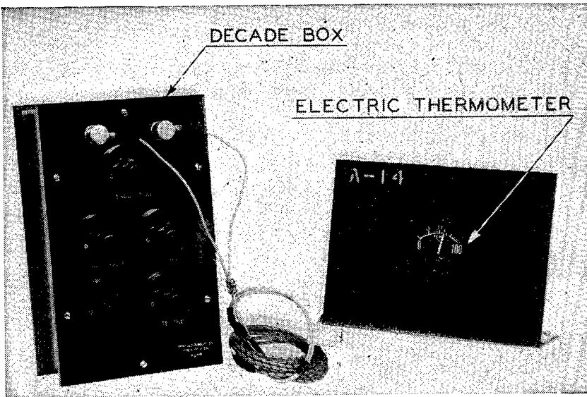
FIGURE 139.—Decade box as used for thermometer test.
