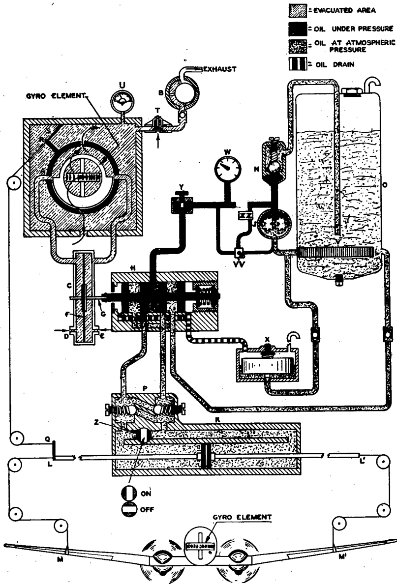
FIGURE 91.—Diagram of automatic pilot showing lateral control only.
