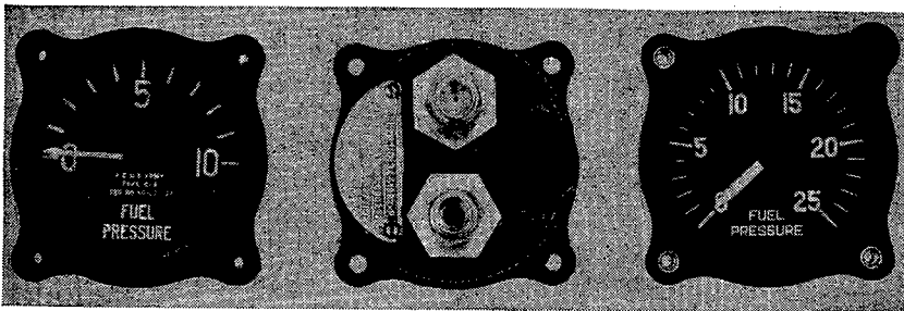
① A-0 to 10-pound gage. ② Rear view. ③ C-0 to 25-pound gage.
