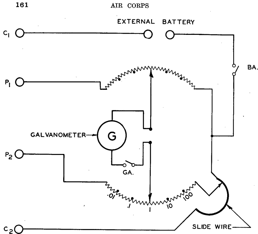
FIGURE 134.—Simplified diagram of Kelvin double bridge.
