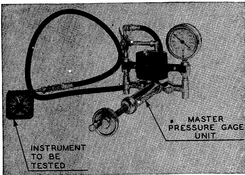
FIGURE 118.—Gage connection to master pressure gage unit.
