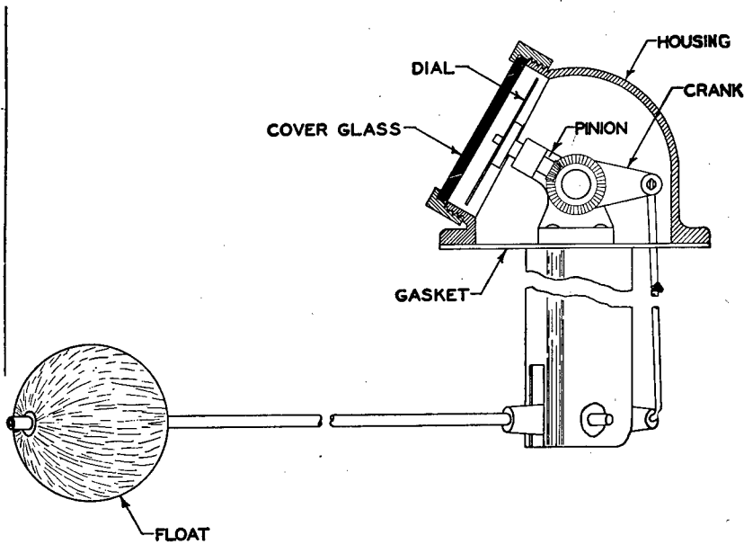
FIGURE 51.—Float and lever type fuel level gage.
