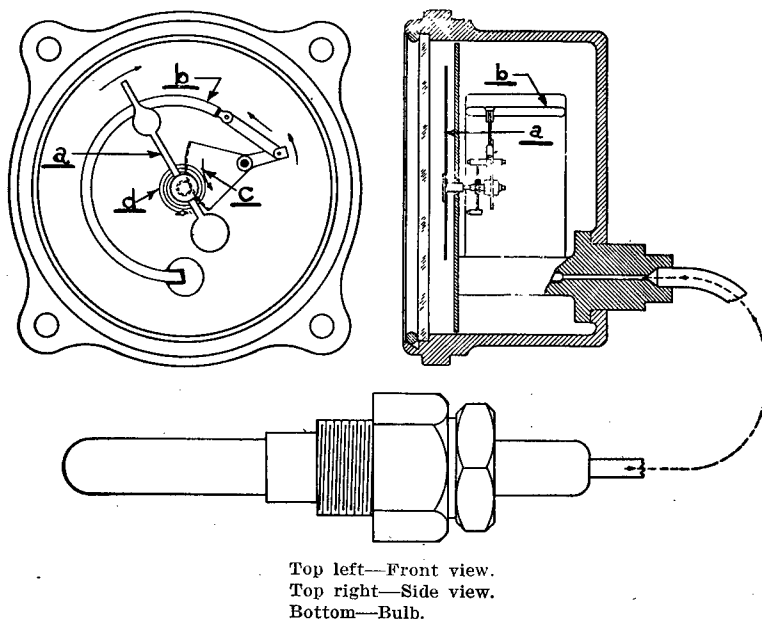
FIGURE 27.—Vapor pressure thermometer mechanism.
