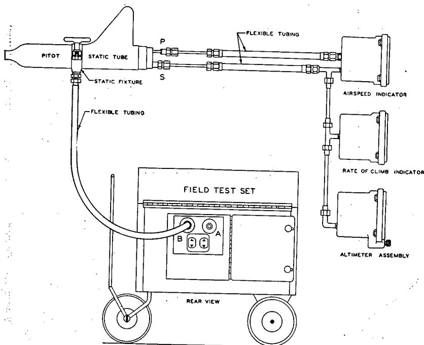
FIGURE 115.—Connection for air speed tube test (static fixture).
