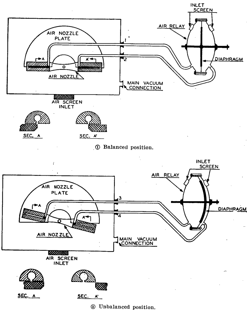
FIGURE 92.—Operation diagrams of air relay and air nozzle.
