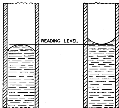
FIGURE 123.—Manometer scales.
