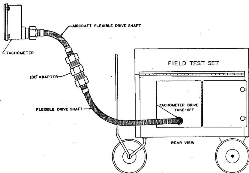
FIGURE 110.—Connection for chronometric tachometer (shaft-driven type) test.
