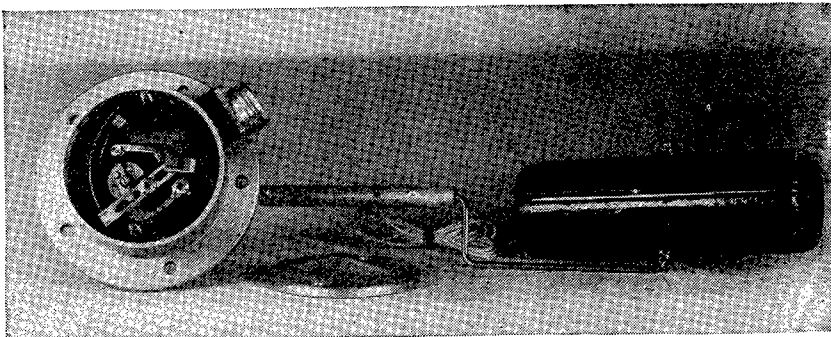
FIGURE 54.—Tank unit of the ratio meter fuel level gage.
