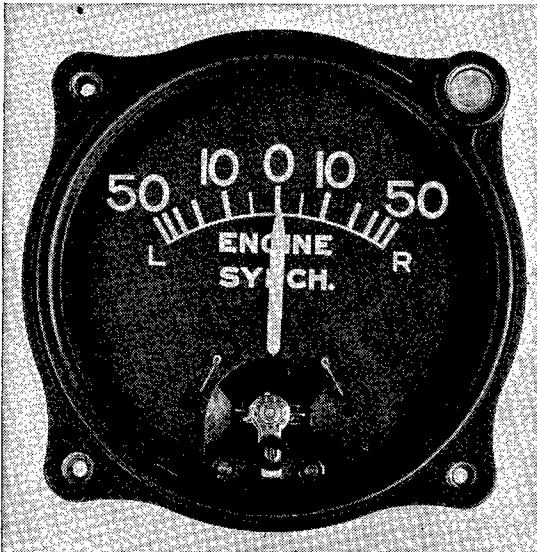
FIGURE 20.—Synchronism indicator.
