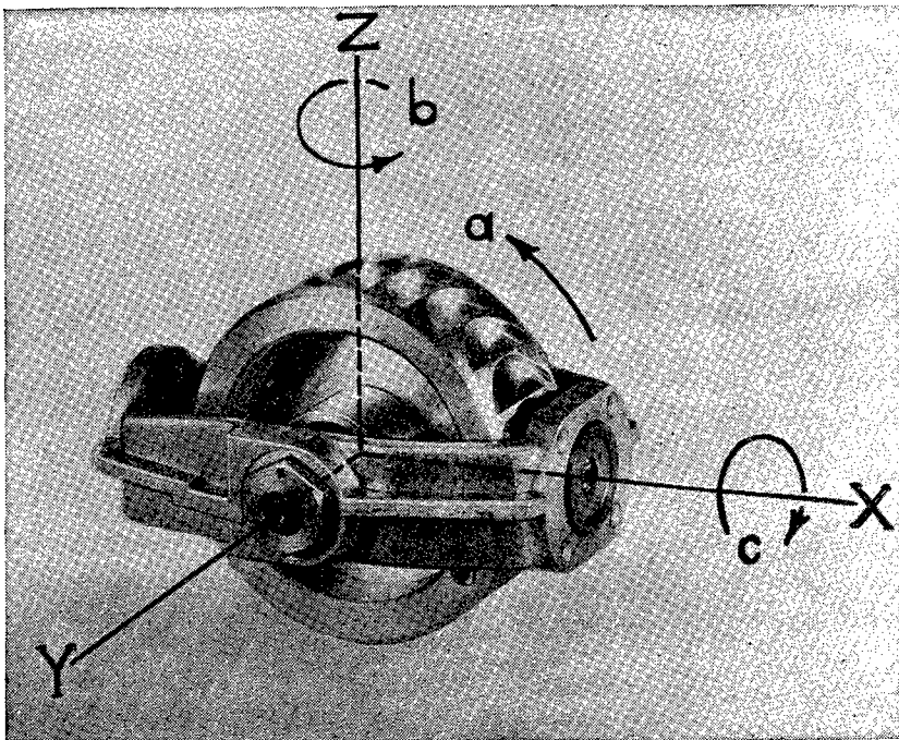
FIGURE 73.—Gyro rotor, bank and turn indicator.
