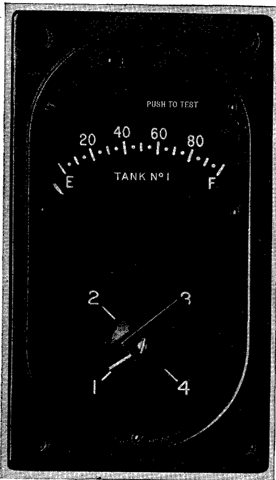
FIGURE 53.—Indicator unit of the ratio meter fuel level gage.
