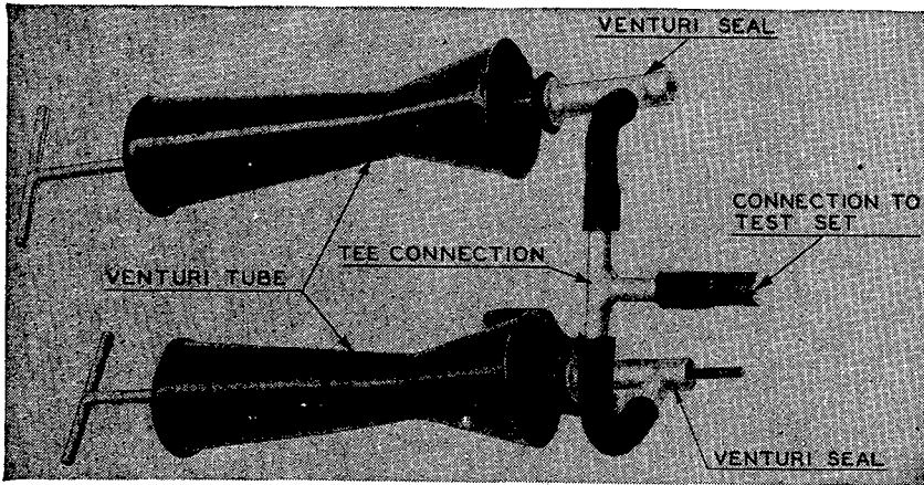
FIGURE 117.—Connection for venturi seals.
