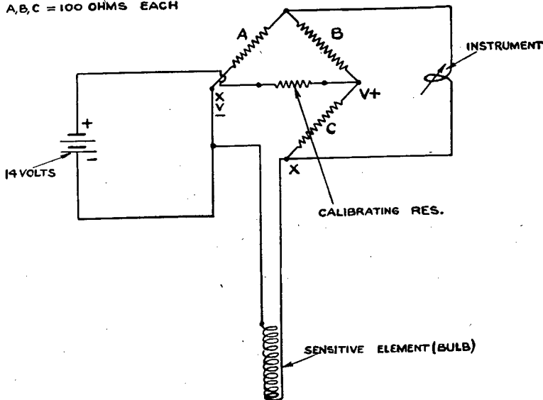
FIGURE 29.—Wiring diagram of electrically operated thermometer.
