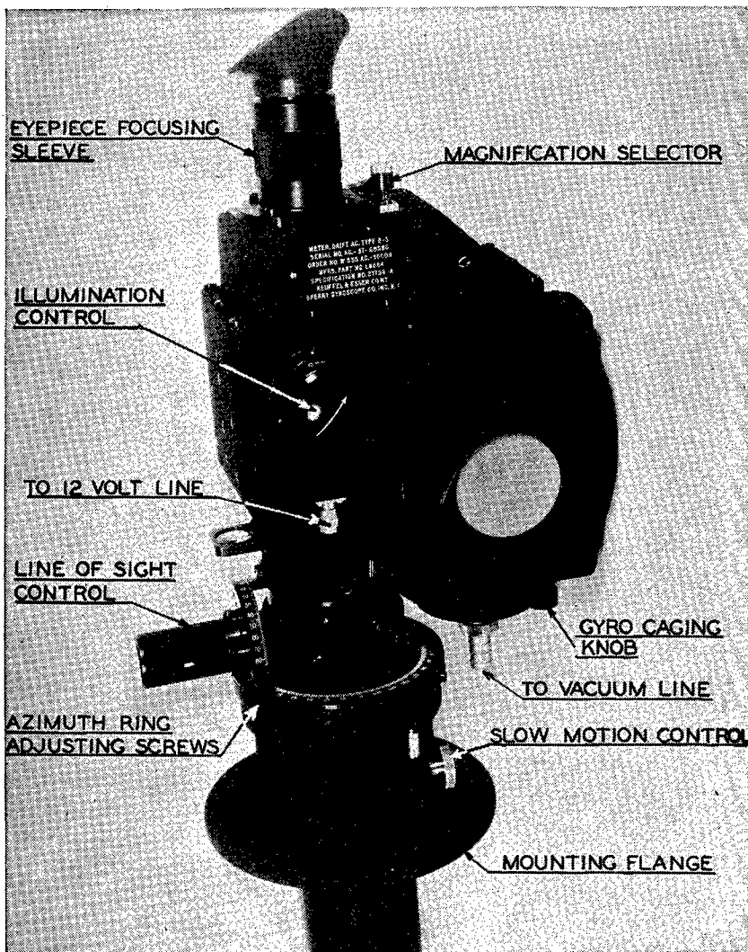
FIGURE 98.—Type B-3 driftmeter.
