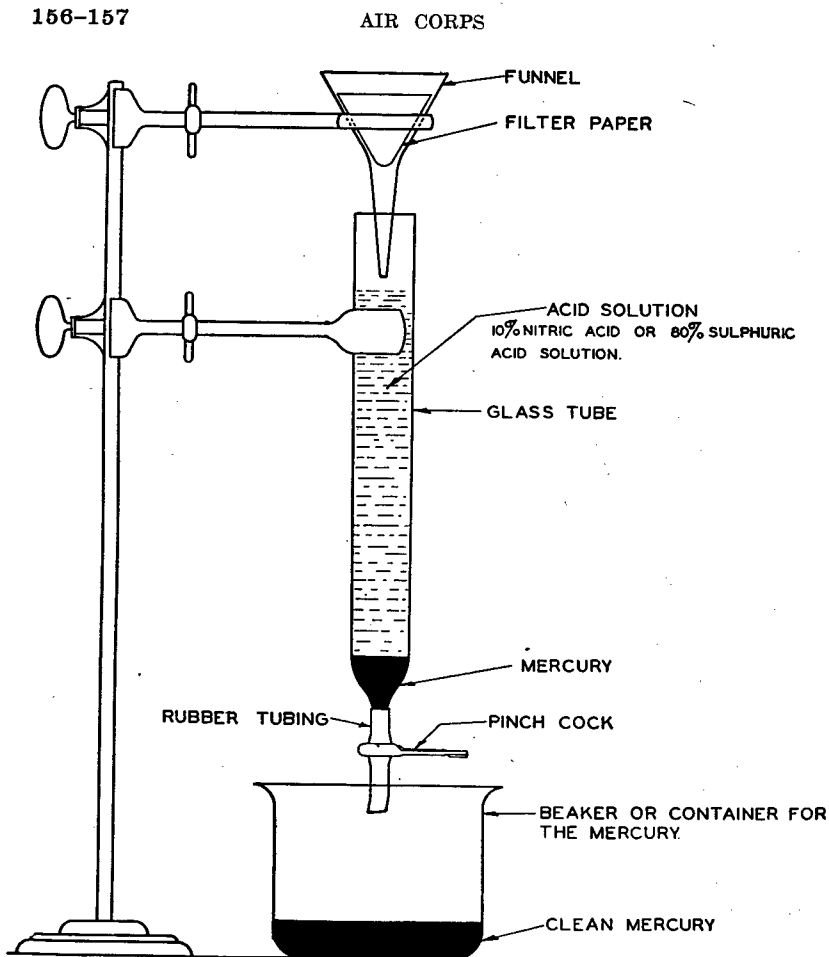
FIGURE 125.—Apparatus for cleaning mercury.
