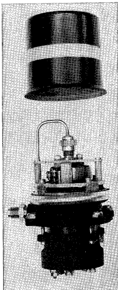
FIGURE 42.—Self-synchronous fuel pressure transmitter.
