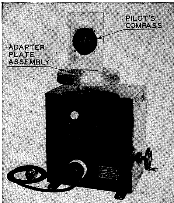
FIGURE 144.—Damping test of pilot's compass.
