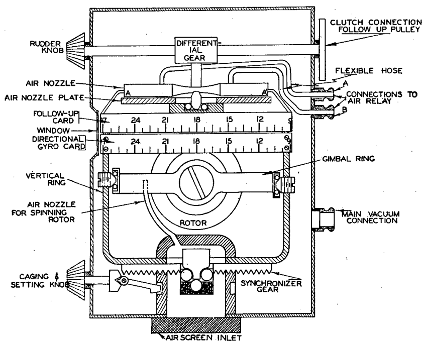
FIGURE 93.—Diagram of air pick-off arrangement, follow-up pulley clutch, and differential gear box.
