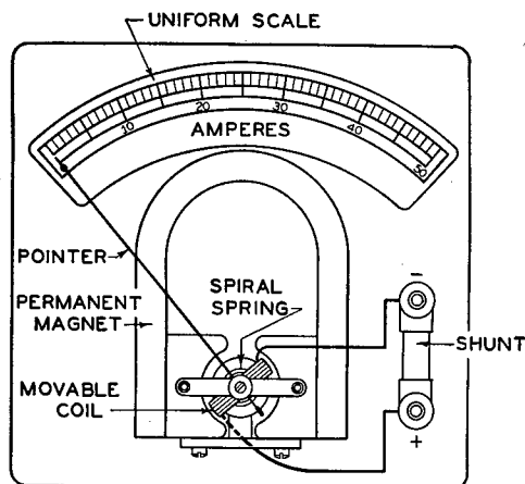
FIGURE 132.—D'Arsonval type ammeter.
