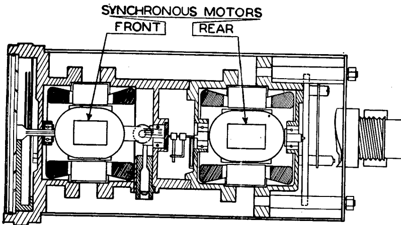
FIGURE 41.—Dual pointer, self-synchronous indicator.
