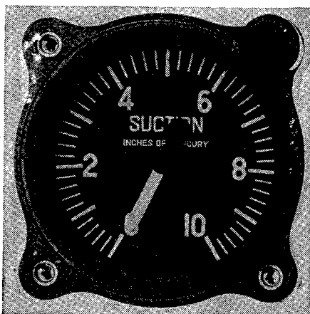
FIGURE 7.—Suction gage.
