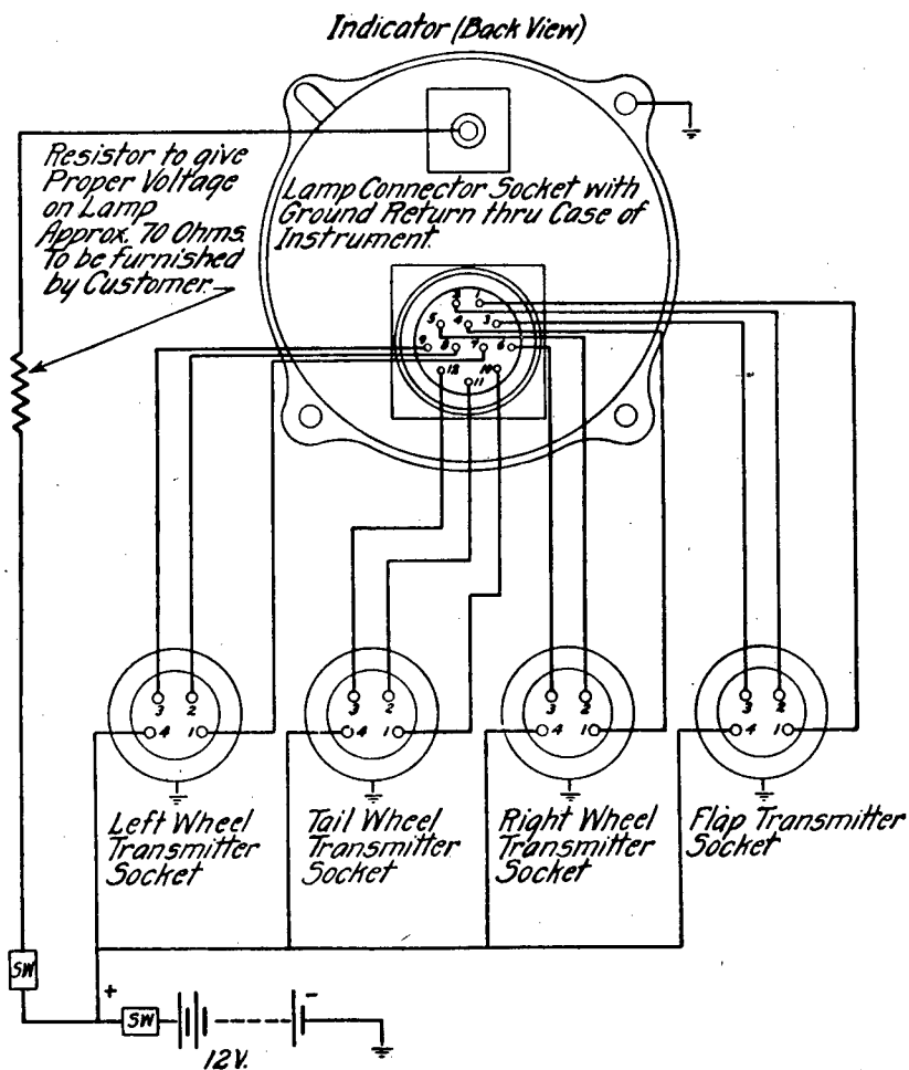
FIGURE 47.—Installation diagram of Selsyn wheel and flap position indicator.
