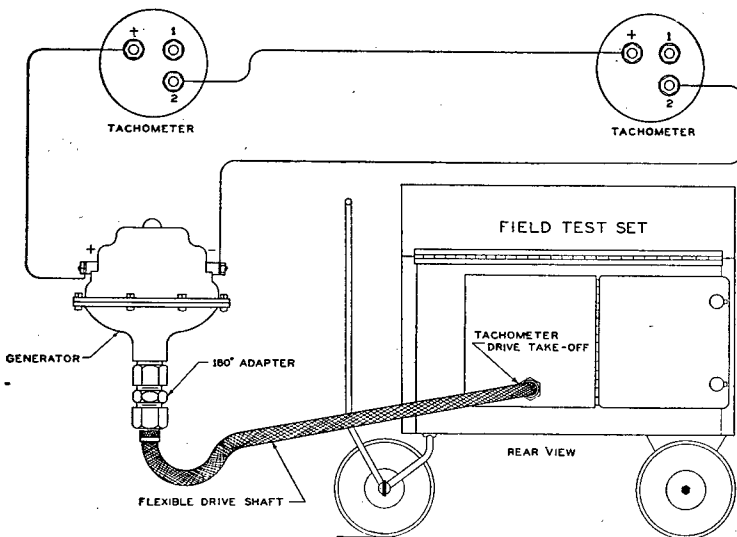
② Dual tachometer indicator installation.
