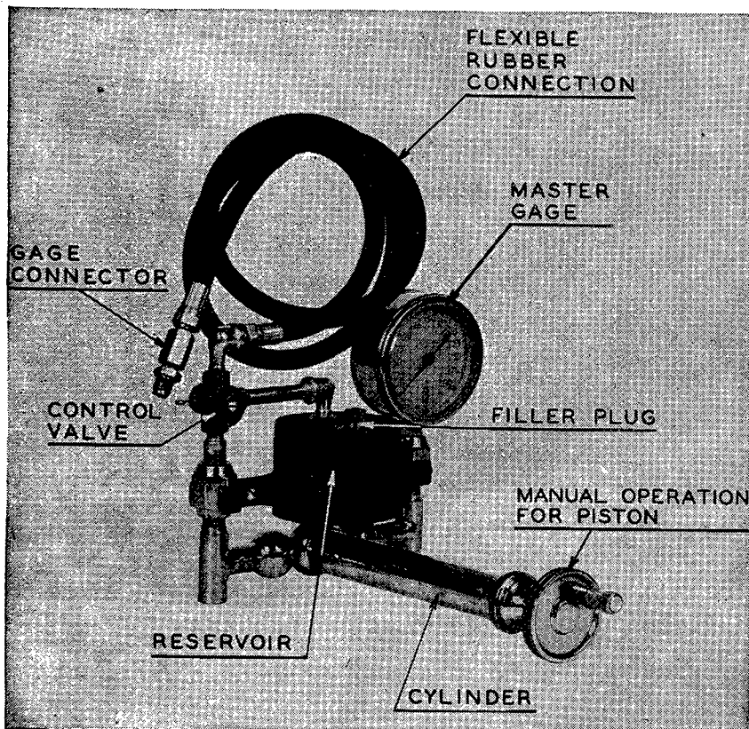
FIGURE 105.—Master pressure gage unit.
