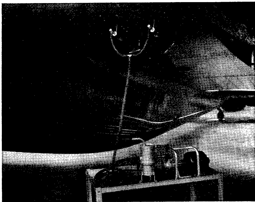
FIGURE 79.—Testing installed gyro instruments using a portable vacuum pump.
