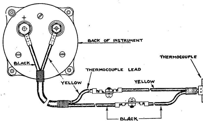
FIGURE 35.—Diagram showing connection of cylinder temperature gage, thermocouple, and leads.
