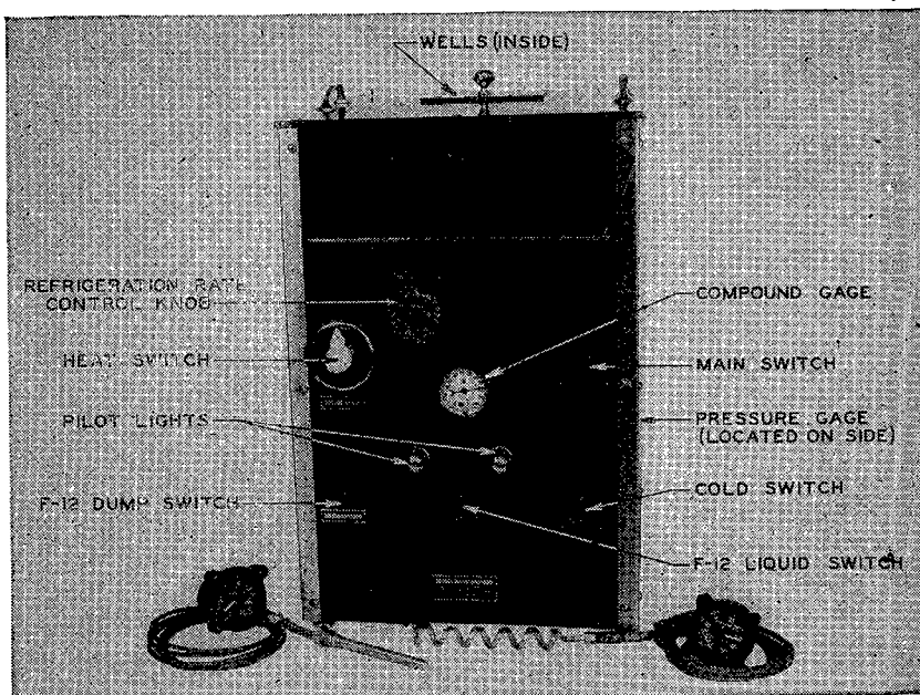
FIGURE 140.—Vapor pressure thermometer tester.
