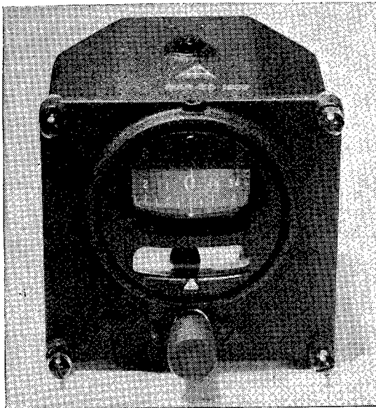
FIGURE 75.—Turn indicator, type A.
