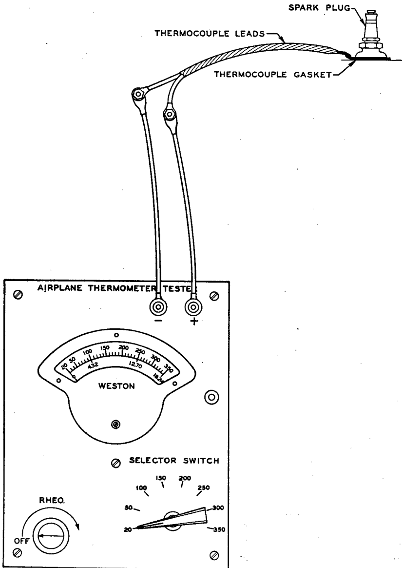
FIGURE 120.—Connection for thermocouple lead resistance test.
