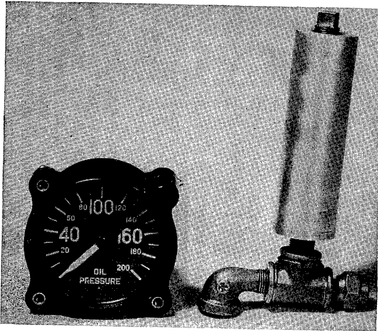
FIGURE 12.—Oil pressure gage and surge chamber.
