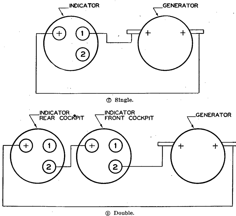
FIGURE 19.—Wiring diagram of generator voltmeter tachometer installation.
