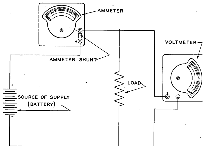
FIGURE 130.—Simple electrical circuit.
