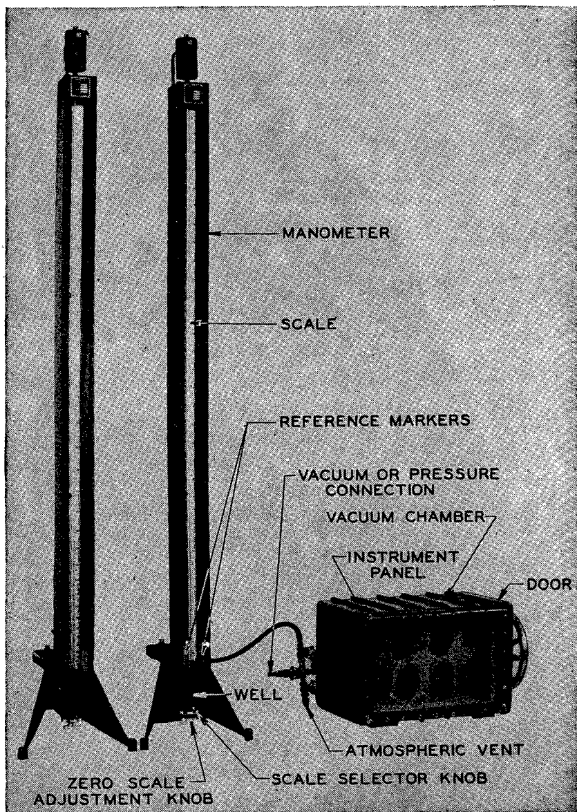
FIGURE 122.—Manometer and vacuum chamber.
