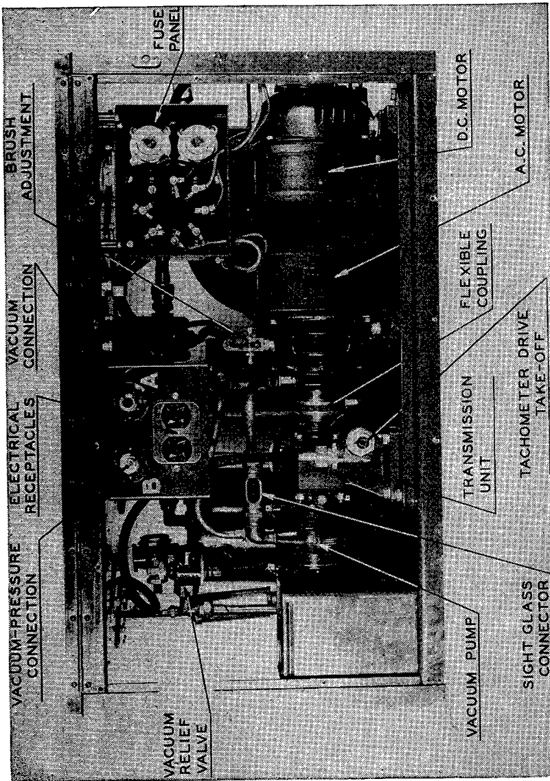
Figure 102.—Type C-1 test set, rear panel removed.
