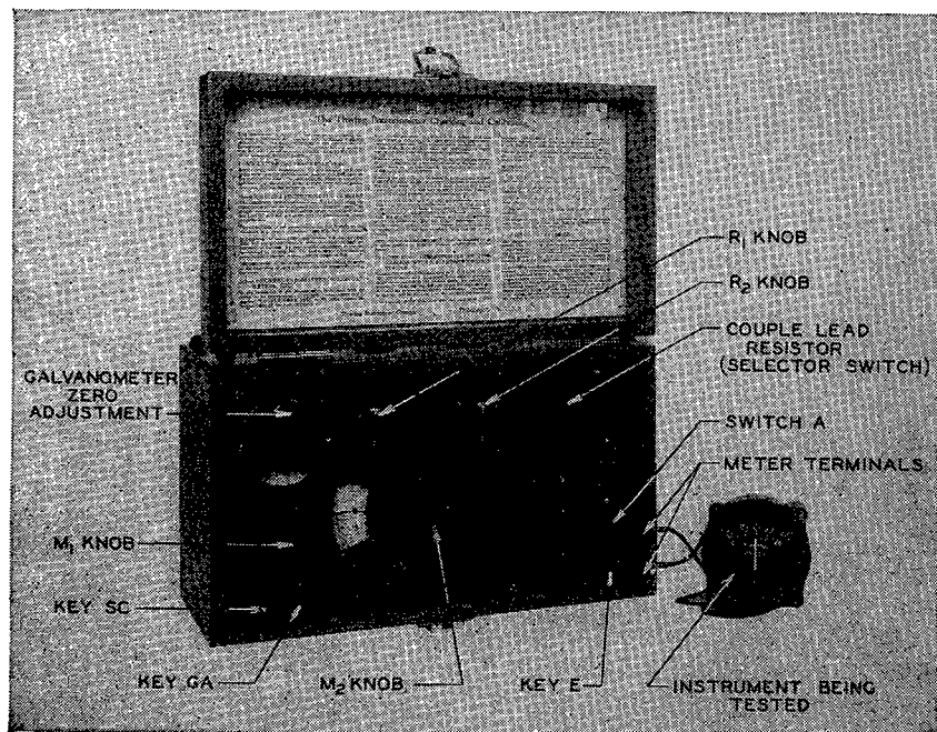
FIGURE 137.—Thwing potentiometer.
