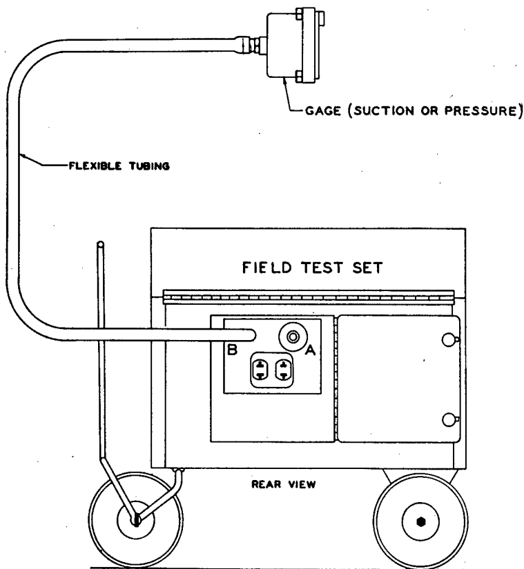
FIGURE 113.—Connection for suction or pressure gage test.
