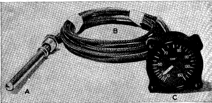
A. Bulb. B. Capillary. C. Indicator.
