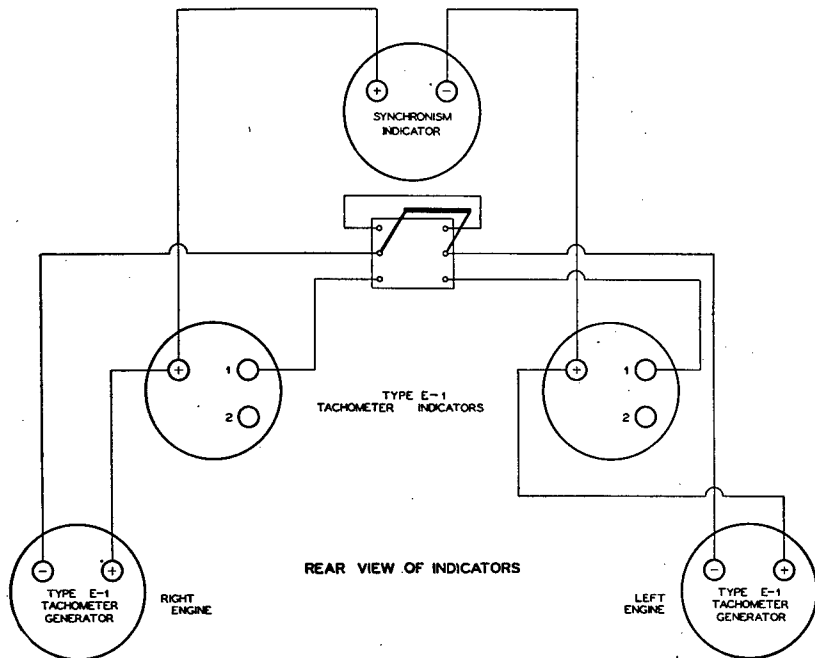
FIGURE 21.—Wiring diagram for installation of generator voltmeter tachometers and synchronism indicators.
