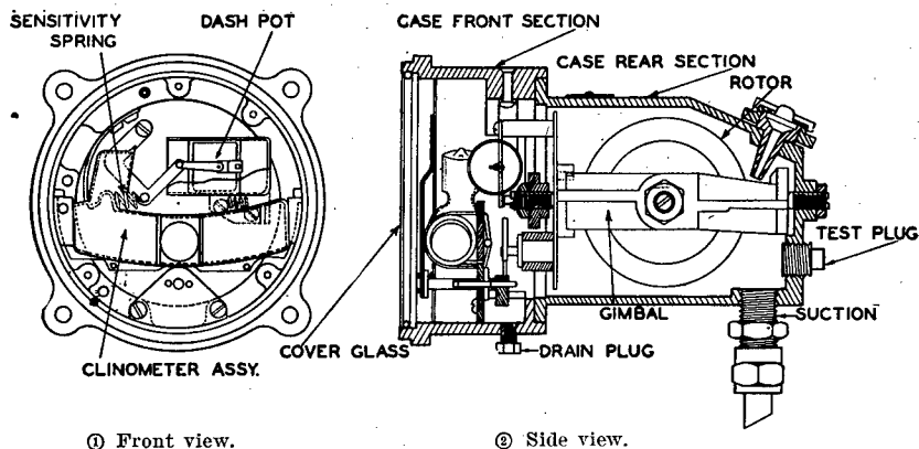
FIGURE 72.—Cross section diagram of the bank and turn indicator.
