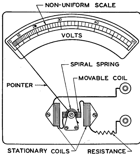
FIGURE 128.—Dynamometer type voltmeter.
