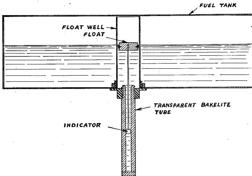
FIGURE 52.—Direct reading float type level gage.
