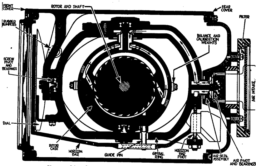
FIGURE 84.—Cross section of flight indicator (top view).
