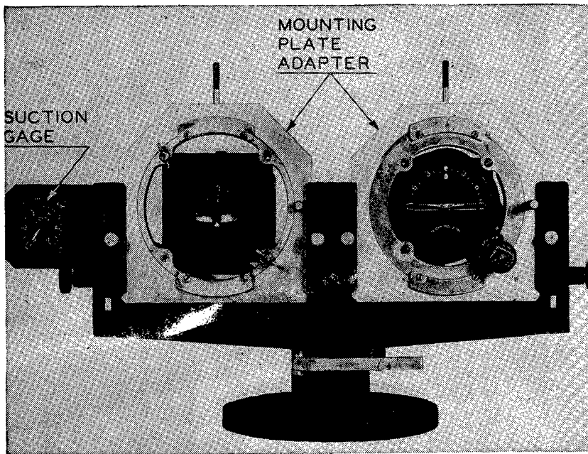
FIGURE 146.—Gyroscopic instrument test fixture.
