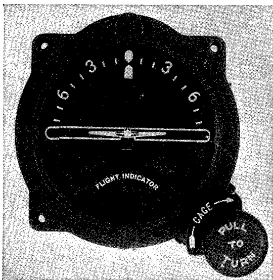
FIGURE 80.—Flight indicator with caging knob (front view).
