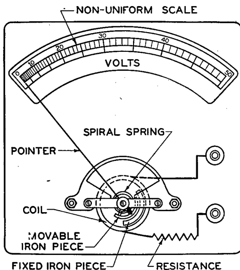
FIGURE 129.—Iron vane-type voltmeter.
