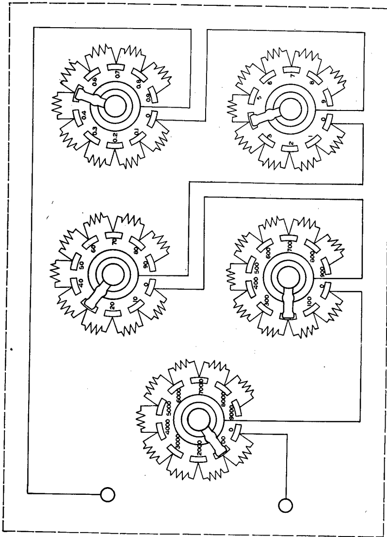
FIGURE 138.—Simplified diagram of decade box.
