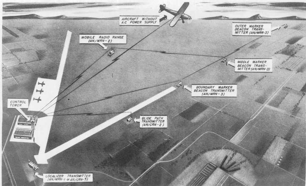
Radio Set SCR-610 is a short range communications equipment used principally for communication between the various transmitters of the AAF Instrument Approach System and the airport control tower.
