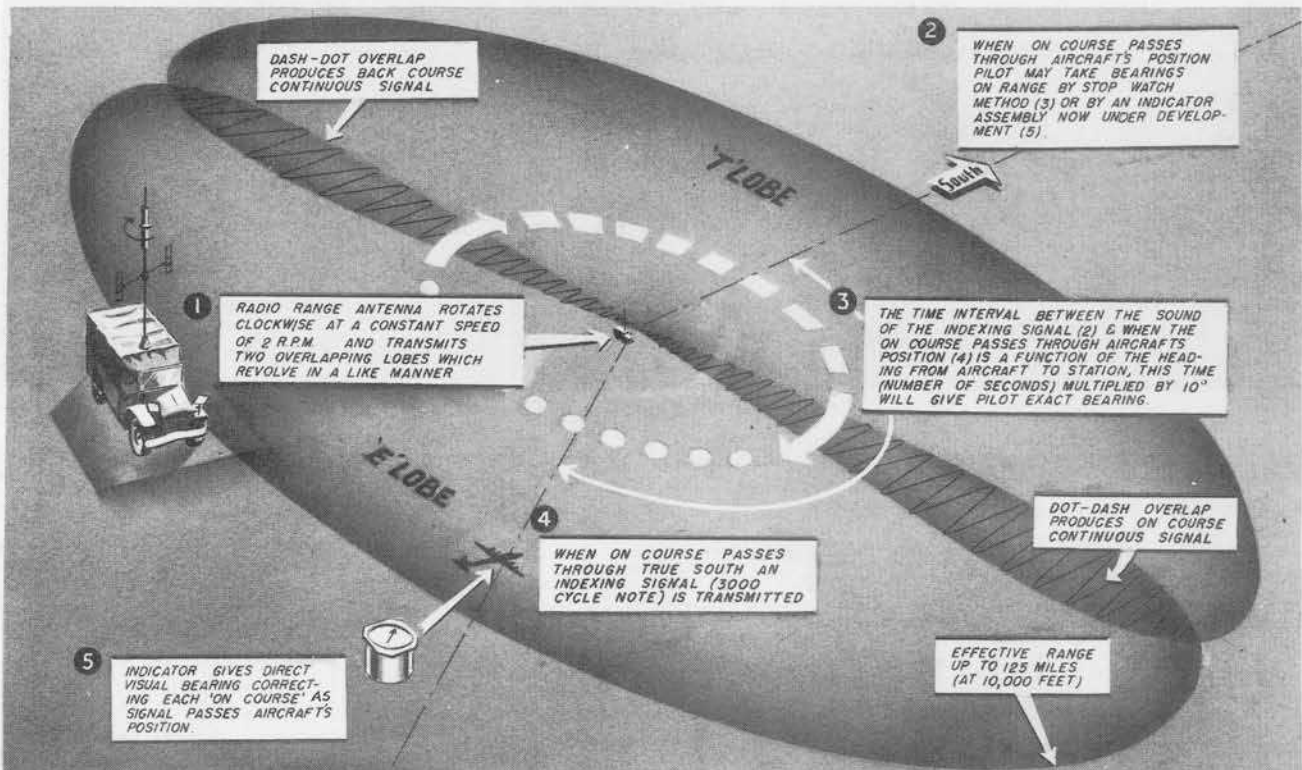
Radio Set SCR-629 (modified) is a mobile VHF omni-directional radio range which enables aircraft to determine relative position with respect to station location and provides periodic station identification and simultaneous voice transmission.
