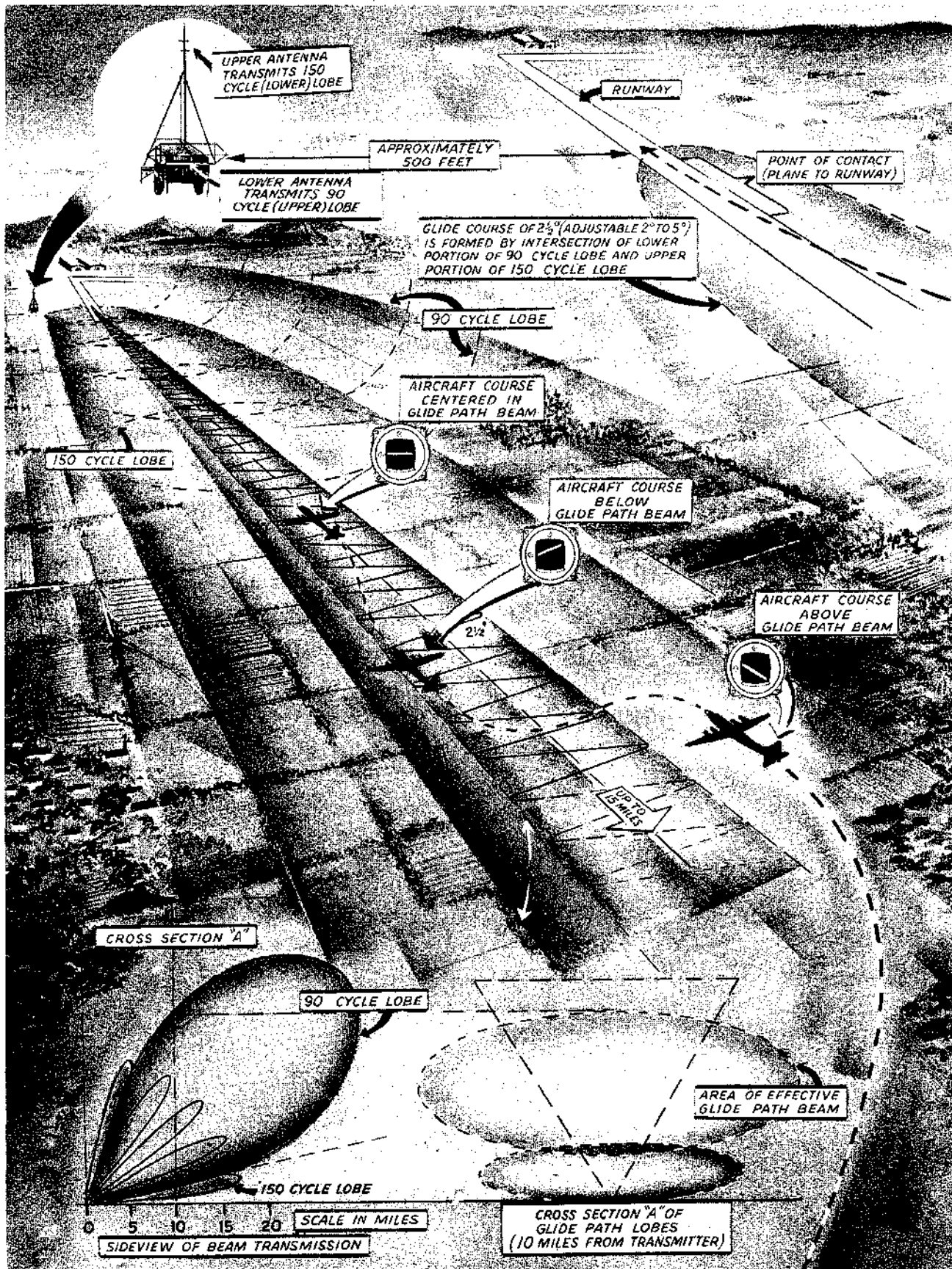
Radió Set AN/CRN-2 is a self contained glide path transmitter, part of the AAF instrument approach system. The glide path beam is obtained by two lobes which intersect and project outward from the runway at an angle of 2\frac{1}{2}^\circ for a distance of approximately 15 miles.
