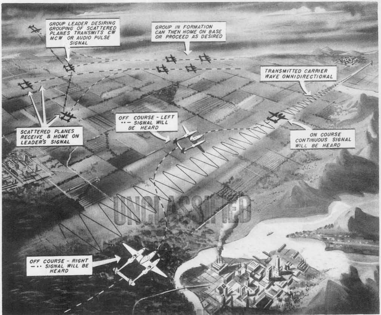
Homing Adapter AN/ARA-8 is used with VHF receivers to provide aircraft with means of homing on any transmitted carrier wave within the frequency range of 120 to 140 mc.
