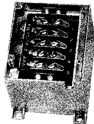
Interior view of Filter F-21/ARA-9 the maintenance of the AN/ARA-9.
