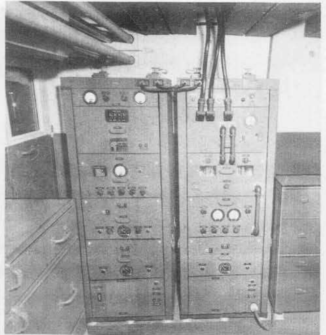
Range Transmitters installed in forward part of truck.
