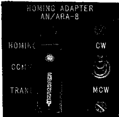
Escutcheon MX-359/ARA-8
