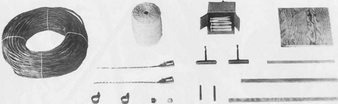
Components of 350 ft. Tow Rope Kit and Tool Kit.
