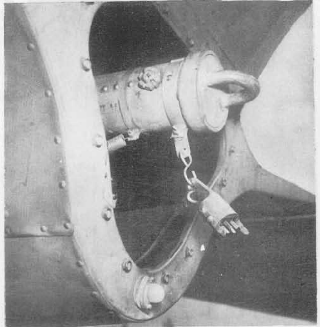
Installation photo showing tow plane connections for AIA-1A.
