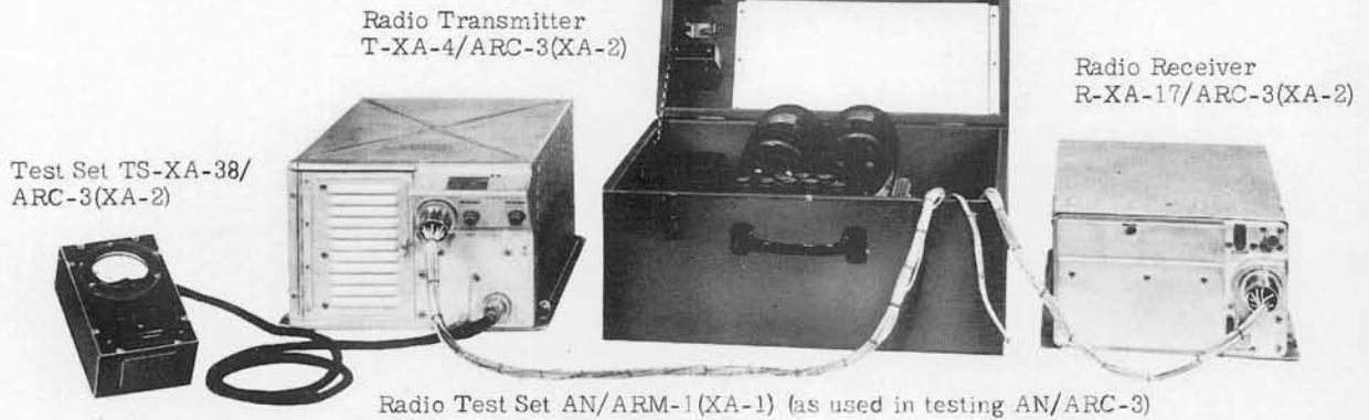
Radio Test Set AN/ARM-1 (as used in testing AN/ARC-3)
