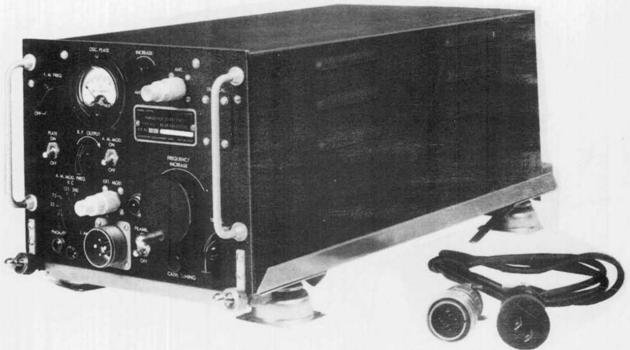
Transceiver RT-54/TPQ-T1
