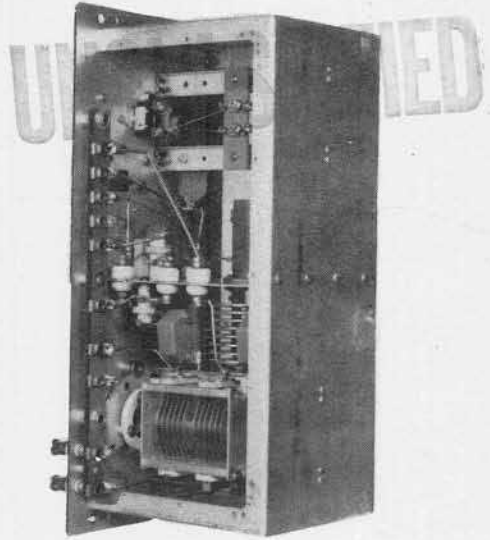
Tuning Unit TU-60
