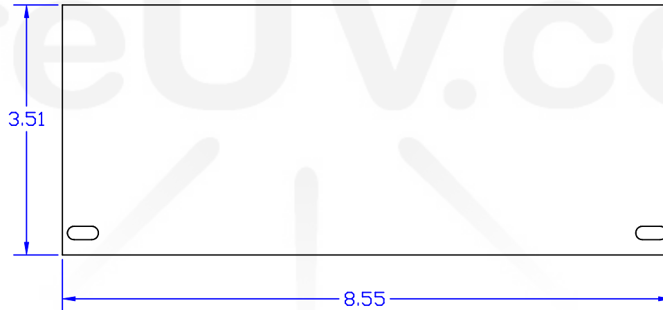
SET CONSISTS OF 2 PIECES ALL DIMENSIONS SHOWN IN FLAT MATERIAL THICKNESS 0.020"
