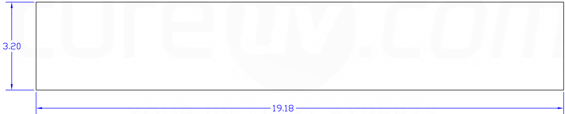
SET CONSISTS OF 2 PIECES ALL DIMENSIONS SHOWN IN FLAT MATERIAL THICKNESS 0.020"
