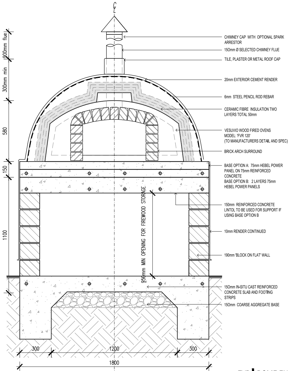
FVR | DOME ENCLOSURE 120 FRONT VIEW
