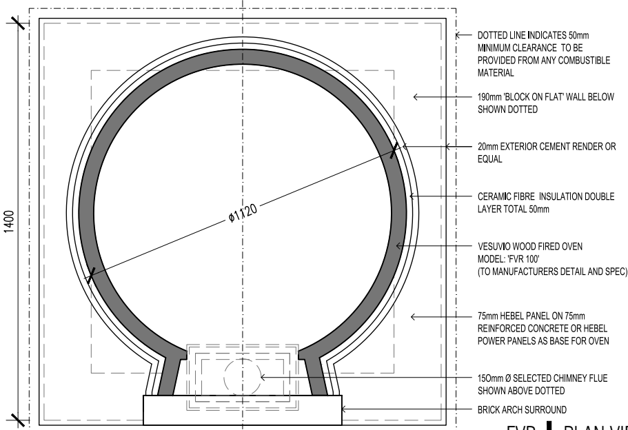
FVR | PLAN VIEW 100
