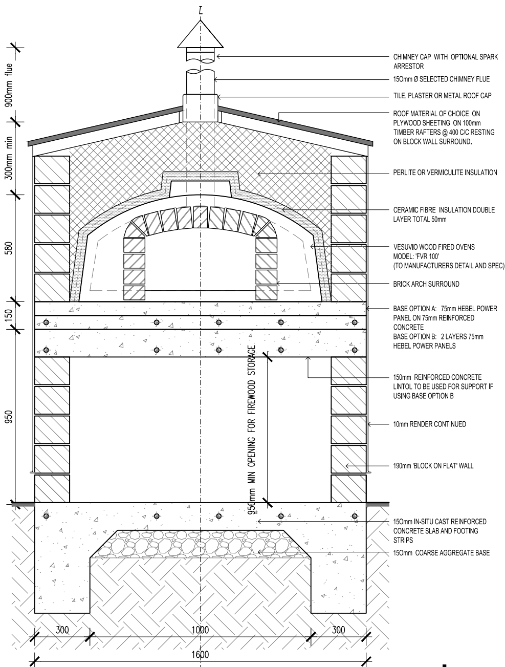
FVR | GABLE ENCLOSURE 100 FRONT VIEW
