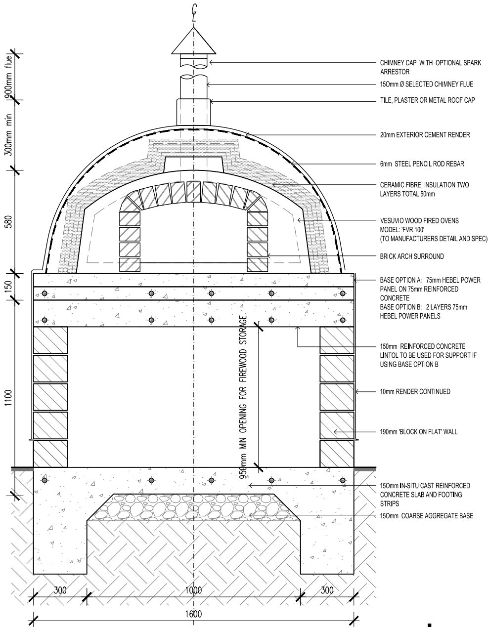
FVR | DOME ENCLOSURE 100 FRONT VIEW
