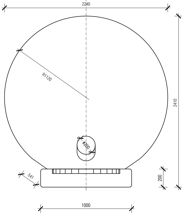
MODEL IGLOO 180 FRONT VIEW
