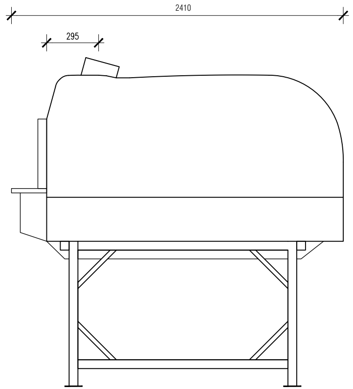
MODEL IGLOO 180 SIDE VIEW
