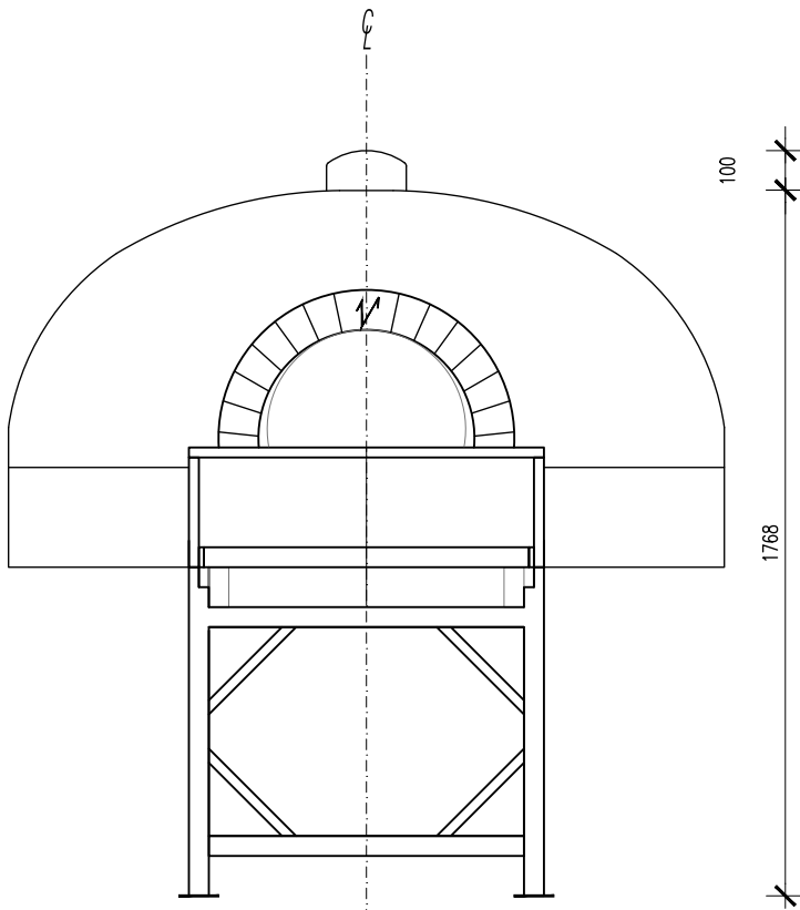
MODEL IGLOO 180 FRONT VIEW
