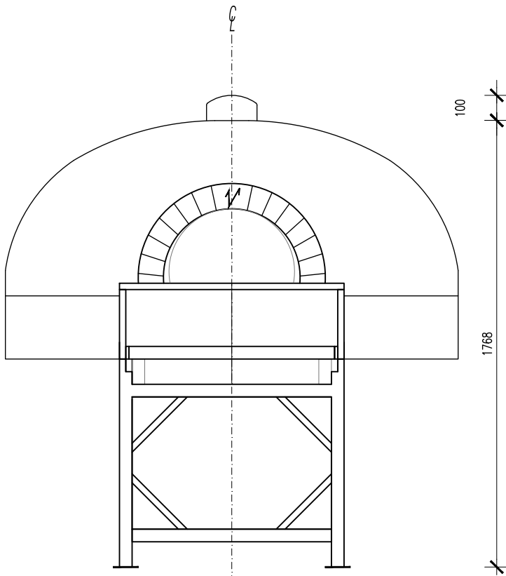
MODEL IGLOO 140 FRONT VIEW
