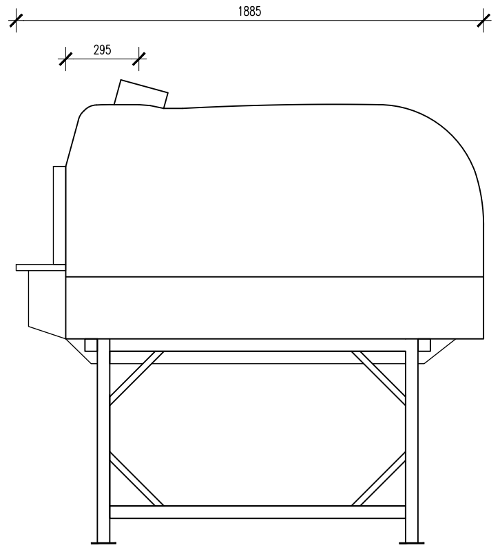
MODEL IGLOO 140 SIDE VIEW
