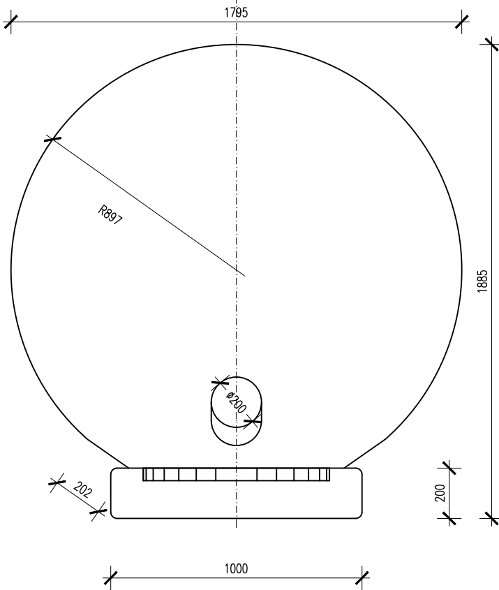
MODEL IGLOO 140 FRONT VIEW
