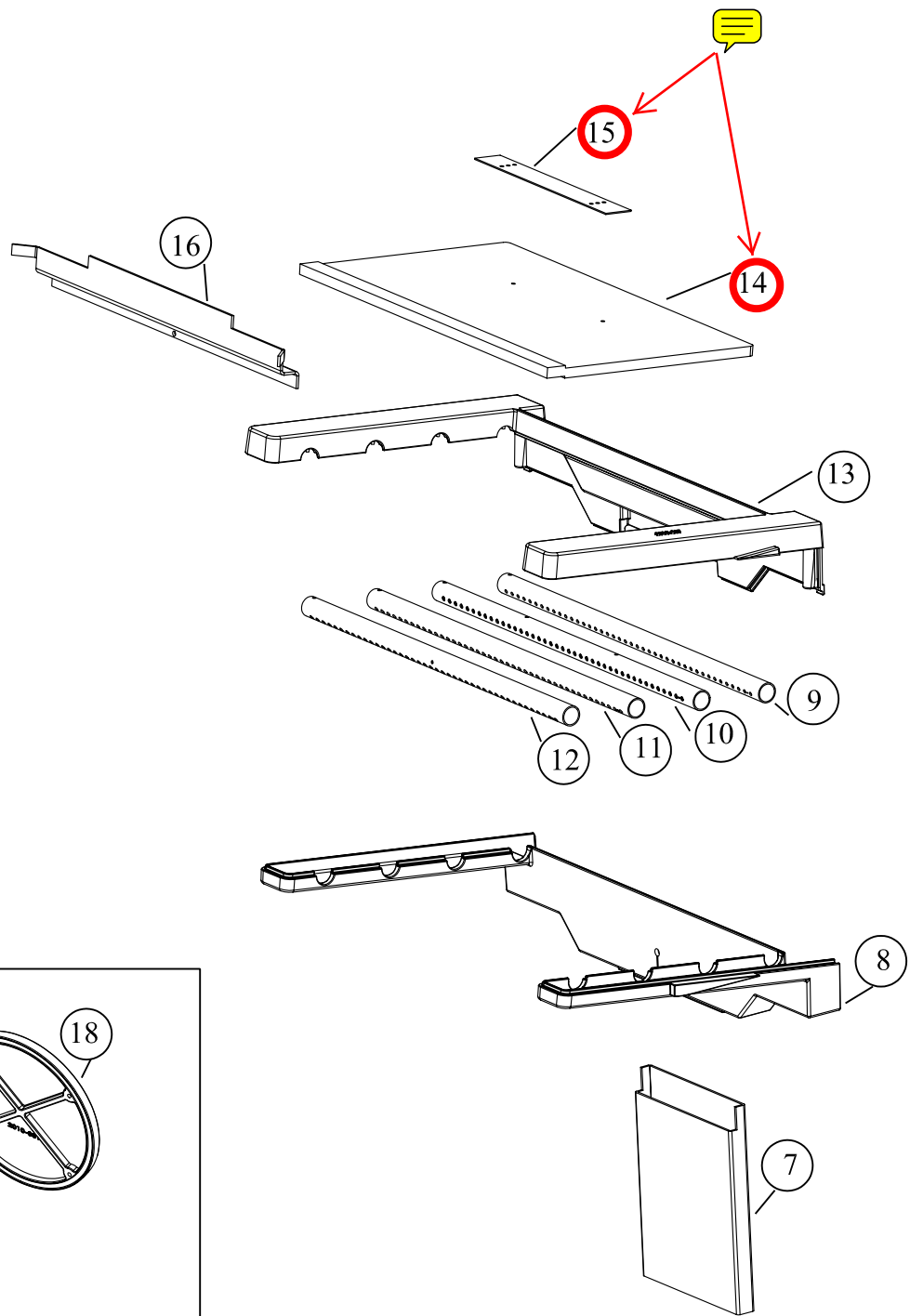
SECONDARY AIR: ASSEMBLY B
