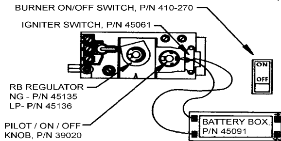
BURNER ON/OFF SWITCH, P/N 410-270
