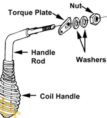
HANDLE ASSEMBLY – P/N 10300
