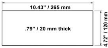
(•11) Upper Rear Firebrick (CI2000HT Series)
