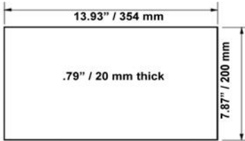
(•12) Left Firebrick (CI1000HT Series)
