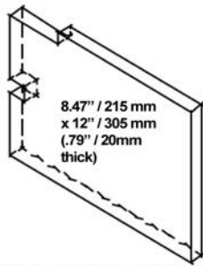
(•13) Lower Rear Firebrick (CI1000HT Series)
