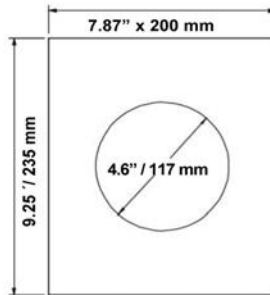
(+5) Bottom Center Firebrick (CI2000HT Series)
