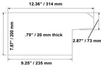
(+6) Bottom Side Firebrick (CI2000HT Series)
