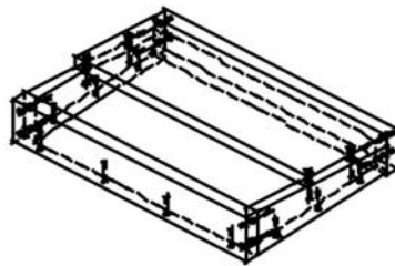
(•38) Start-up Air Channel Assembly (CI2000HT Series)
