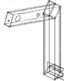
(•31) Right Air Column Assembly (CI1000HT Series)
