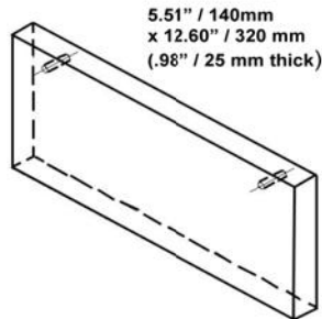
(•16) Upper Rear Firebrick (CI1000HT Series)
