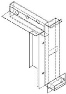
(•33) Upper Air Deflector (CI1000HT Series)
