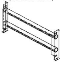
(+44) Secondary Air Tube Assembly (CI2000HT Series)
