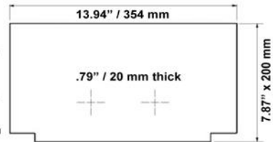
(+9) Lower Rear Firebrick (CI2000HT Series)
