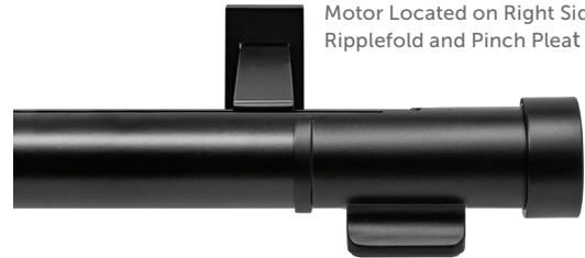
Ceiling Mounted Motor Located on Right Side of Track Ripplefold and Pinch Pleat
