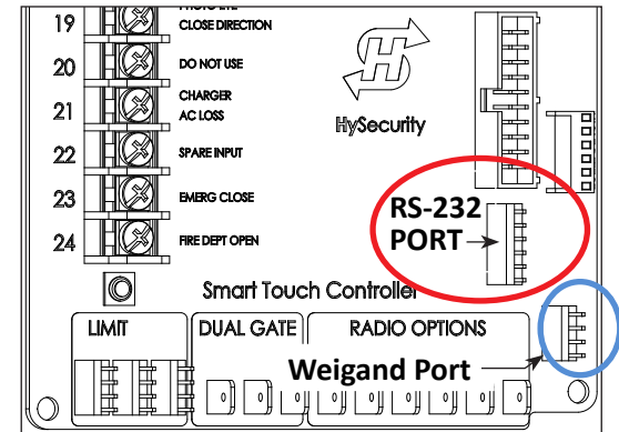
STC New Generation Board HySecurity Hydraulic Operators
