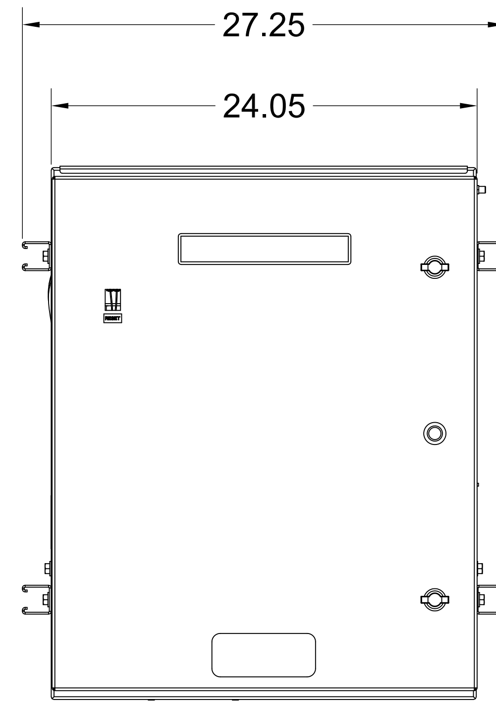
FRONT VIEW
