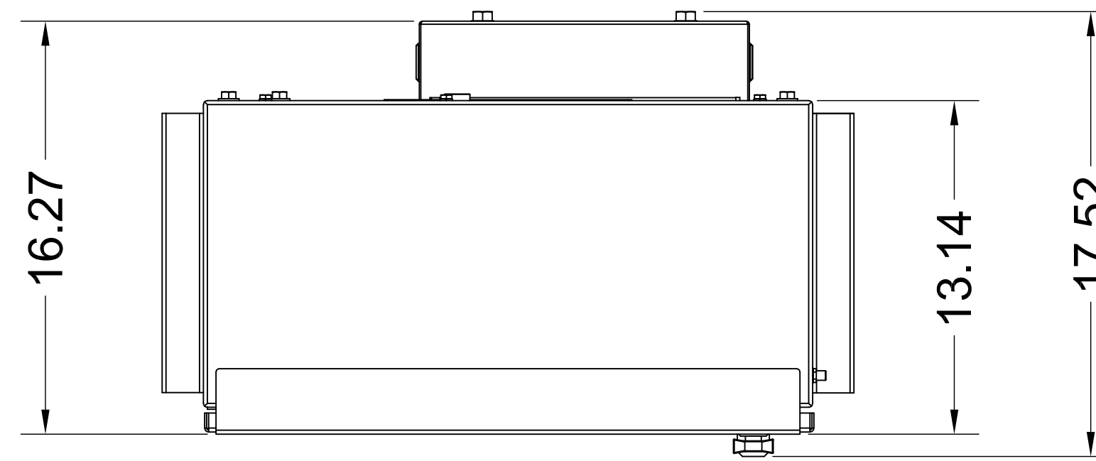
TOP VIEW
