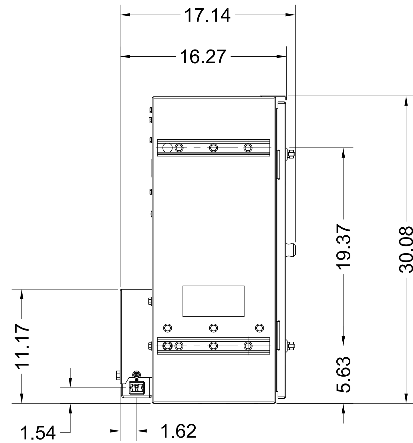
LEFT VIEW
