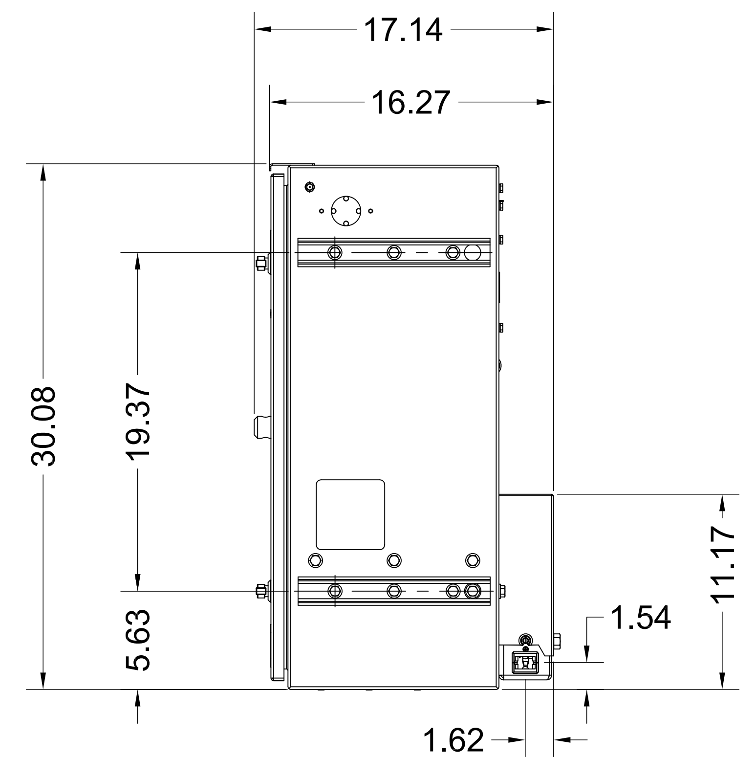
RIGHT VIEW
