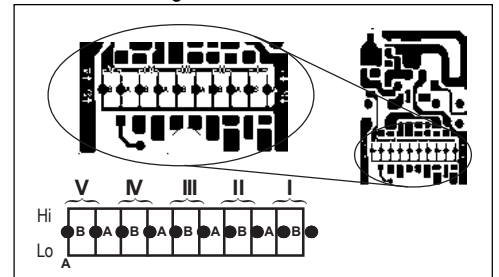
Fig. 1: SK-919TD1S-U / SK-919TD2A-U Series PCB Diagram.
