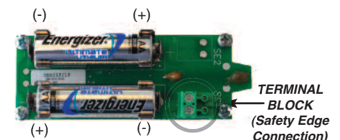
Fig. 2-6 WIRE CONNECTION TO TERMINAL BLOCK
