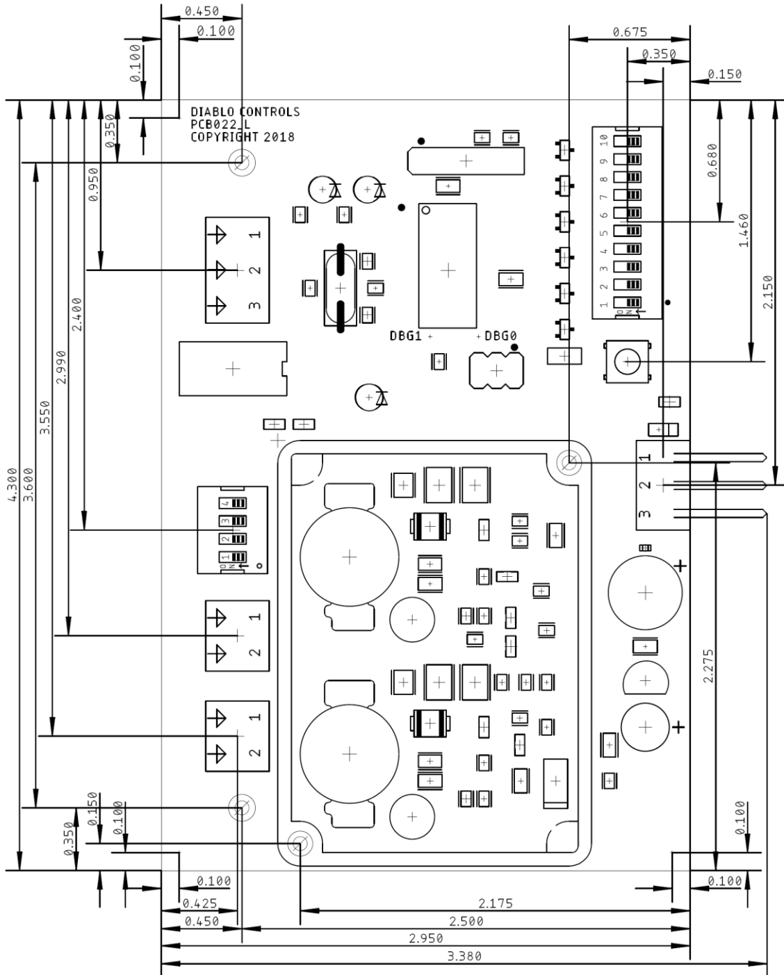
Figure 2: Physical Dimensions
