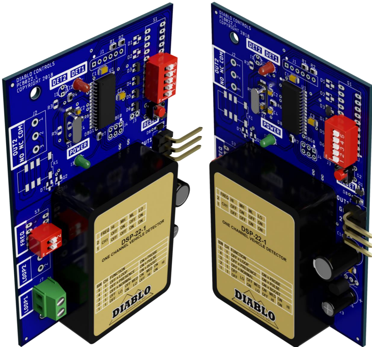
Figure 1: Product Views
