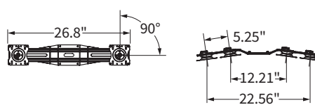
Dual Monitor Adaptor option
