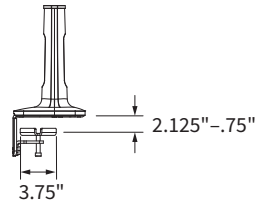
Base C-Clamp
