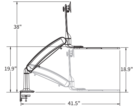
Base reach & range (side)
