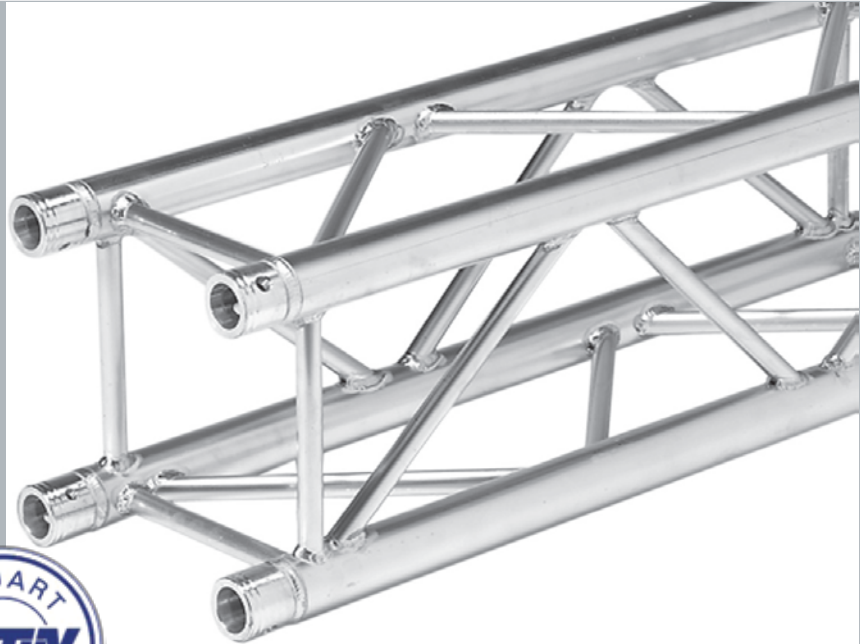
MEGATRUS 290 mm (11.42 in.) 12 inch nominal square section trussing
