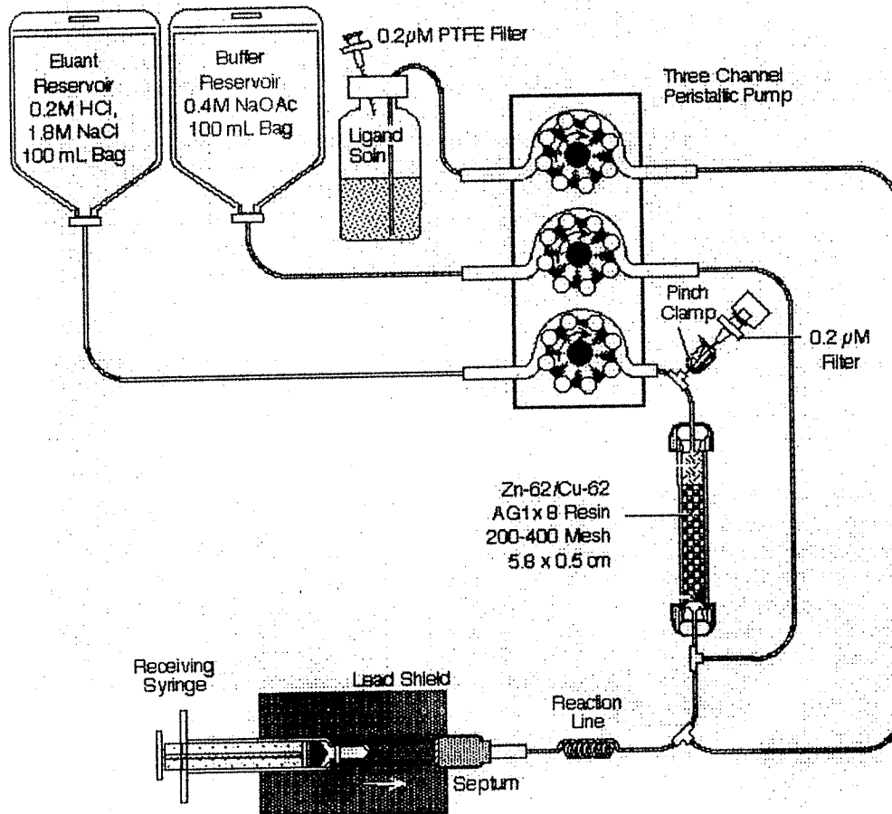
FIGURE 2. Schematic diagram illustrating plumbing of Proportional Technologies ^{62}\text{Zn}/^{62}\text{Cu} generator configured for on-line synthesis and delivery of ^{62}\text{Cu} -PTSM. Final ^{62}\text{Cu} -radiopharmaceutical was consistently delivered at >95\% radiochemical purity into syringe at outlet of generator housing. Integrated steps of generator elution and in-line radiopharmaceutical synthesis require \sim 33 sec.
