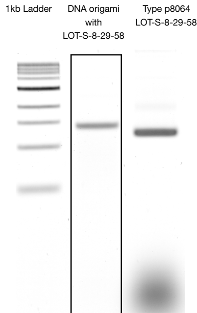
Photograph of an GelRed® stained 2% agarose gel on which purified scaffold DNA samples were electrophoresed.
