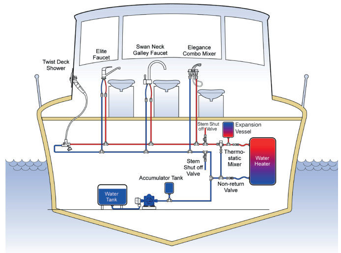
Typical Installation
