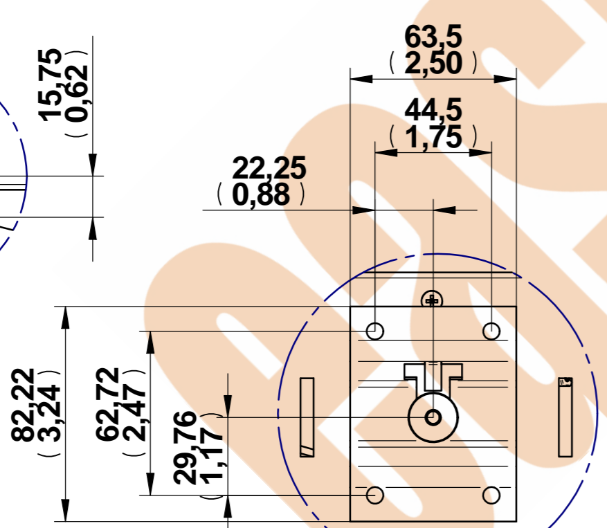
GIMBLE PLATE DETAIL 1:2
