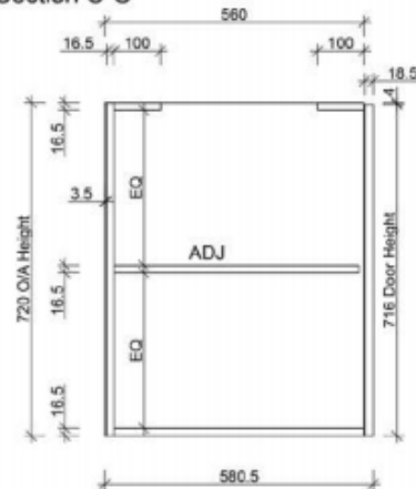
Section C-C
