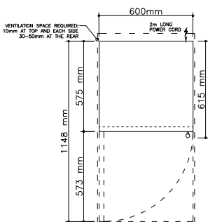
Floor plan
