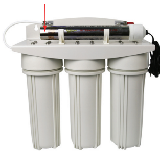
Triple Undersink with a 1 GPM Ultraviolet Water Sterilizer System CQE-US-00325
