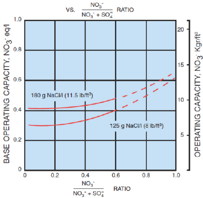
Fig. 5 OPERATING CAPACITY
