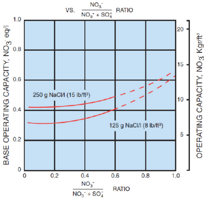
Fig. 3 OPERATING CAPACITY
