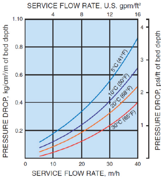
Fig. 1 PRESSURE DROP CHARACTERISTICS
