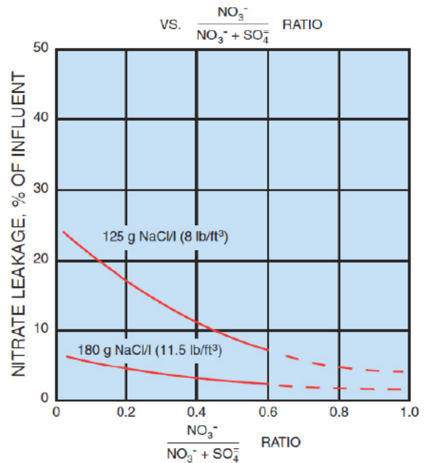
Fig. 6 NITRATE LEAKAGE
