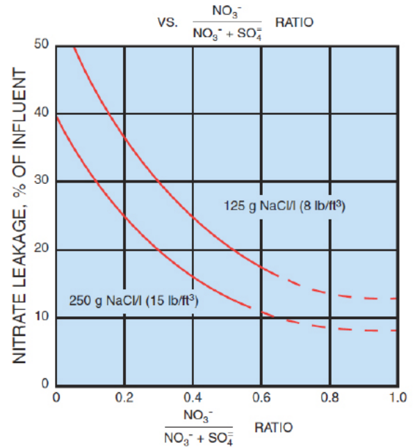
Fig. 4 NITRATE LEAKAGE
