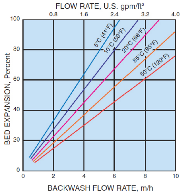
Fig.2 BACKWASH EXPANSION
