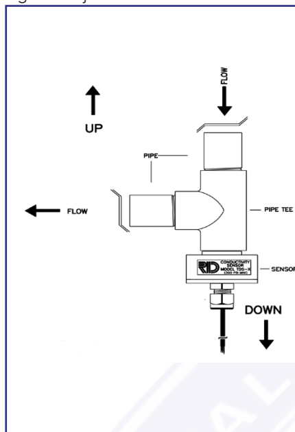
TDS / Conductivity Sensor Installation
