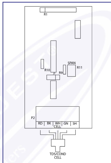
TDS / Conductivity Expander
