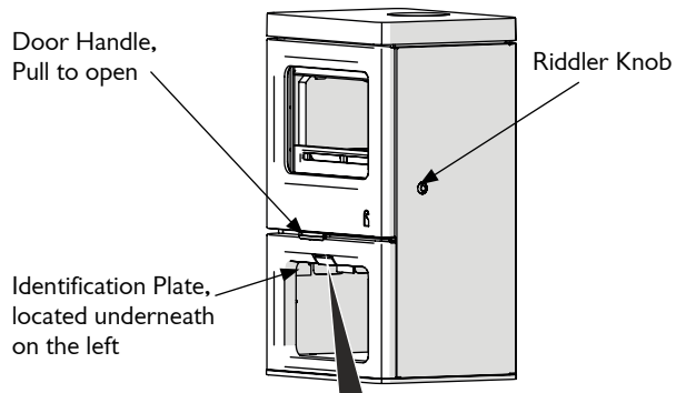
Fig. 3 Stove controls
