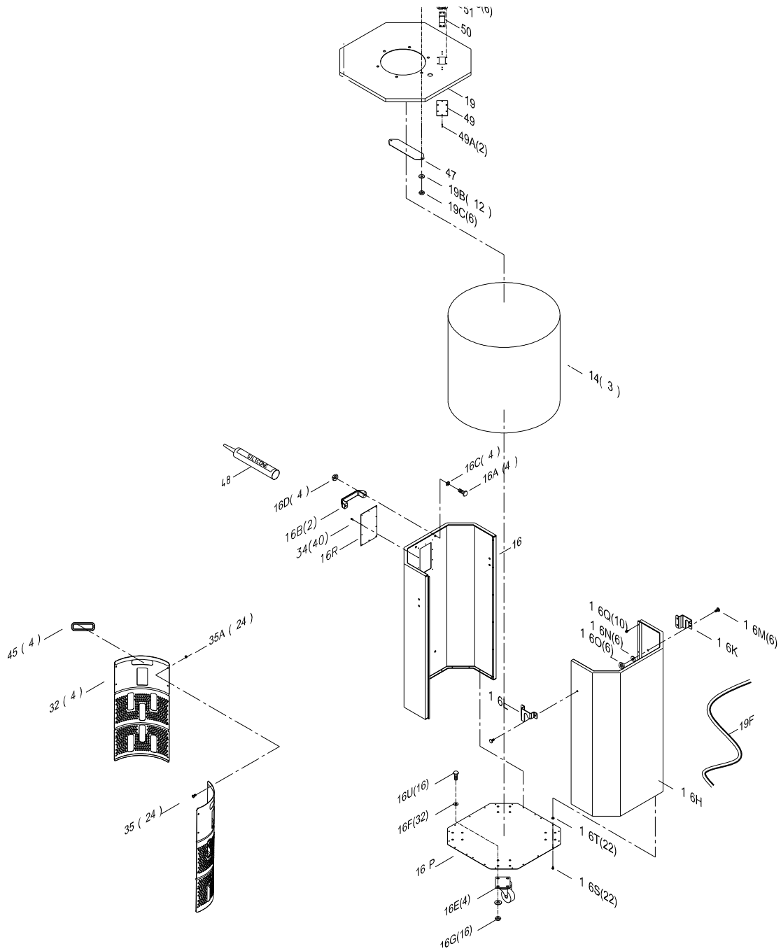
Figure 51: Barrel & insert
