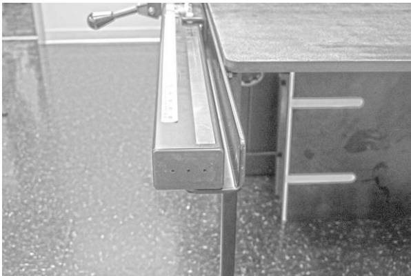
Front guide rail seated on front rail:
