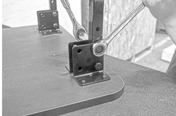
Securing Bolts
