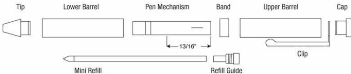
Diagram C - Assembly
