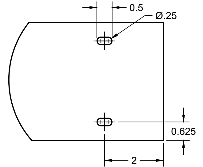
DETAIL A SLOT PATTERN
