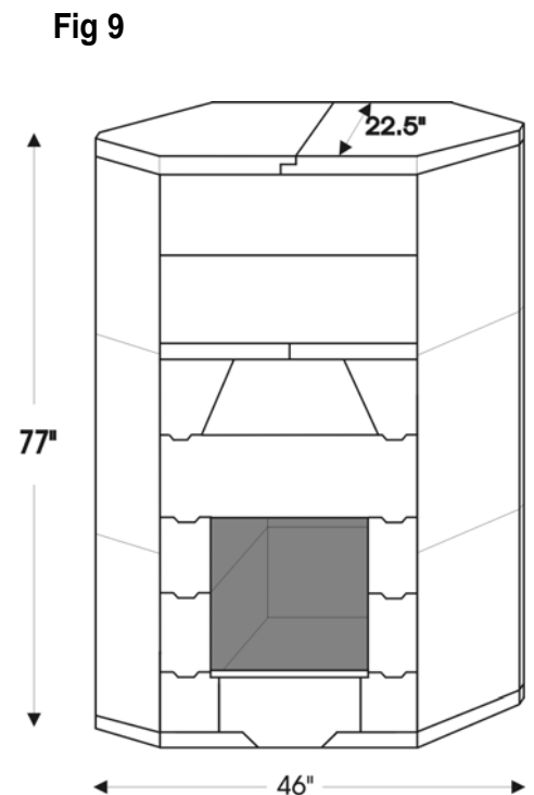
Temp-Cast 2000 (Standard Corner Fireplace)
