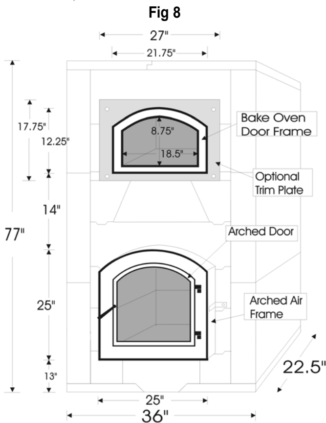
Temp-Cast 2000 Standard Fireplace (with Arched Door & Bake Oven options)
