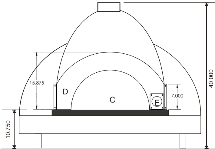
FRONT ELEVATION
