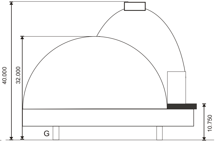
SECTION
